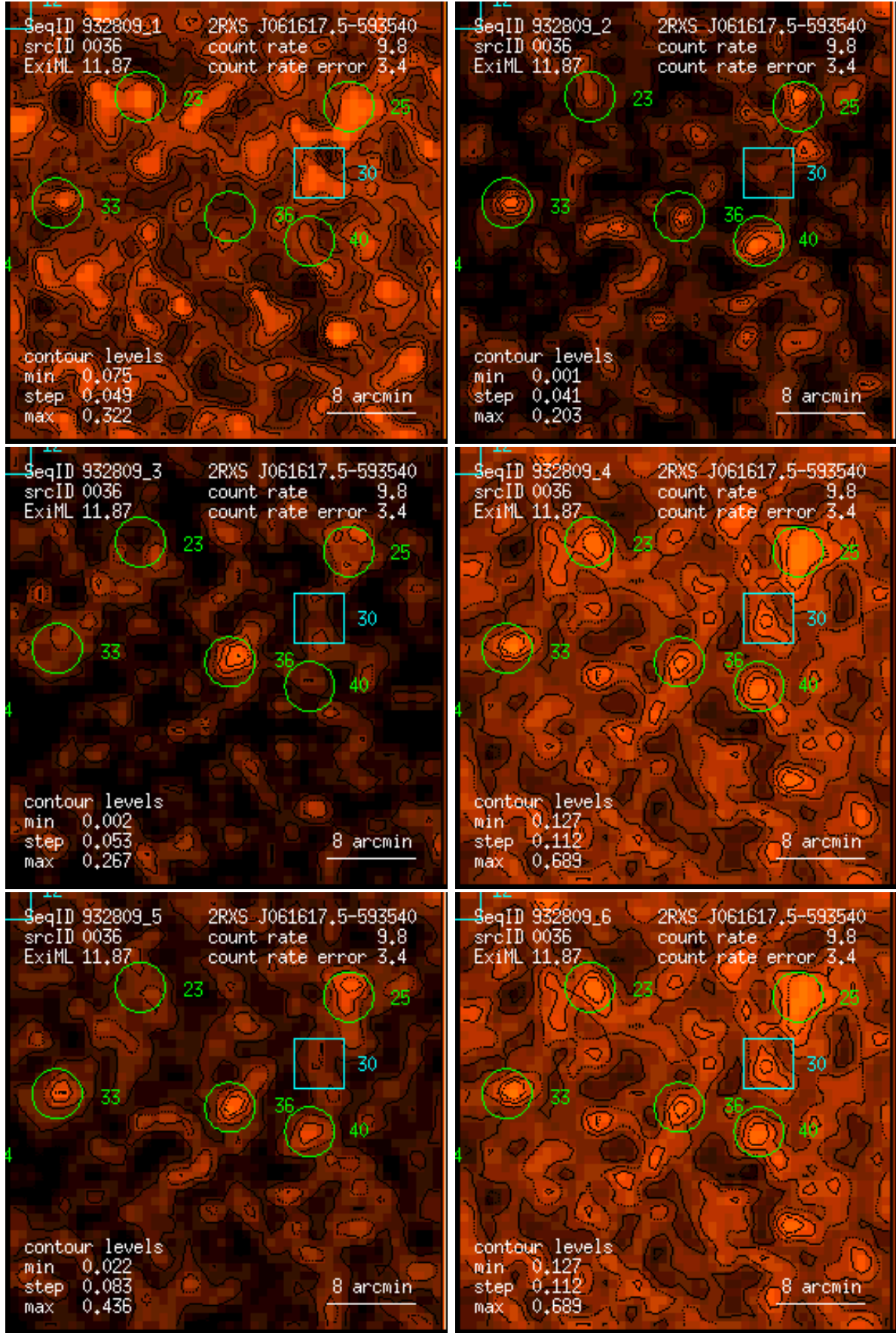
Figure 36: RASS 932809: detection 0036: band rate images, Gaussian filter: (1) PSPC channels 11 – 41, (2) 52 – 90, (3) 91 – 201, (4) 11 – 235, (5) 52 – 201, (6) 11 – 201. Broad band rates in counts/ks. Band rate contour levels in counts/ks/arcmin 2 .
