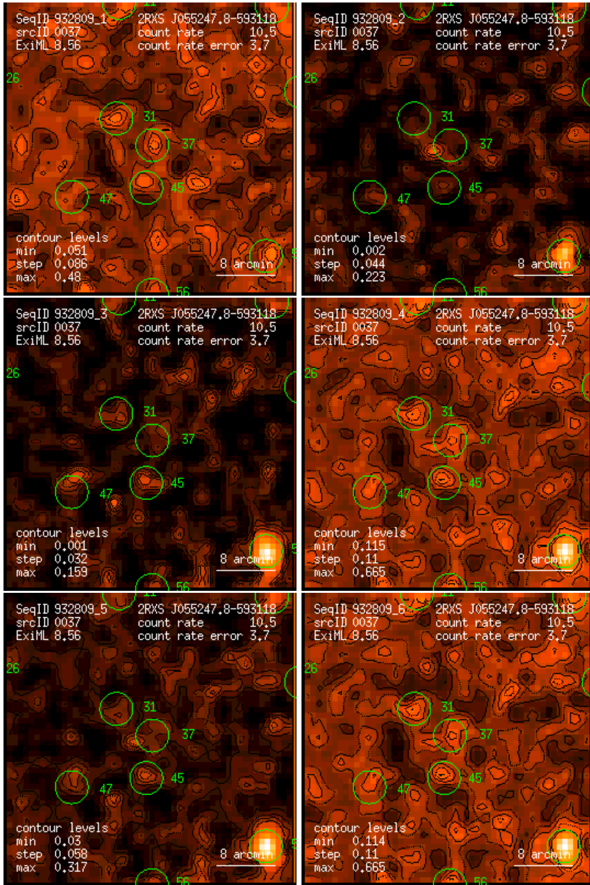
Figure 37: RASS 932809: detection 0037: band rate images, Gaussian filter: (1) PSPC channels 11 – 41, (2) 52 – 90, (3) 91 – 201, (4) 11 – 235, (5) 52 – 201, (6) 11 – 201. Broad band rates in counts/ks. Band rate contour levels in counts/ks/arcmin 2 .
