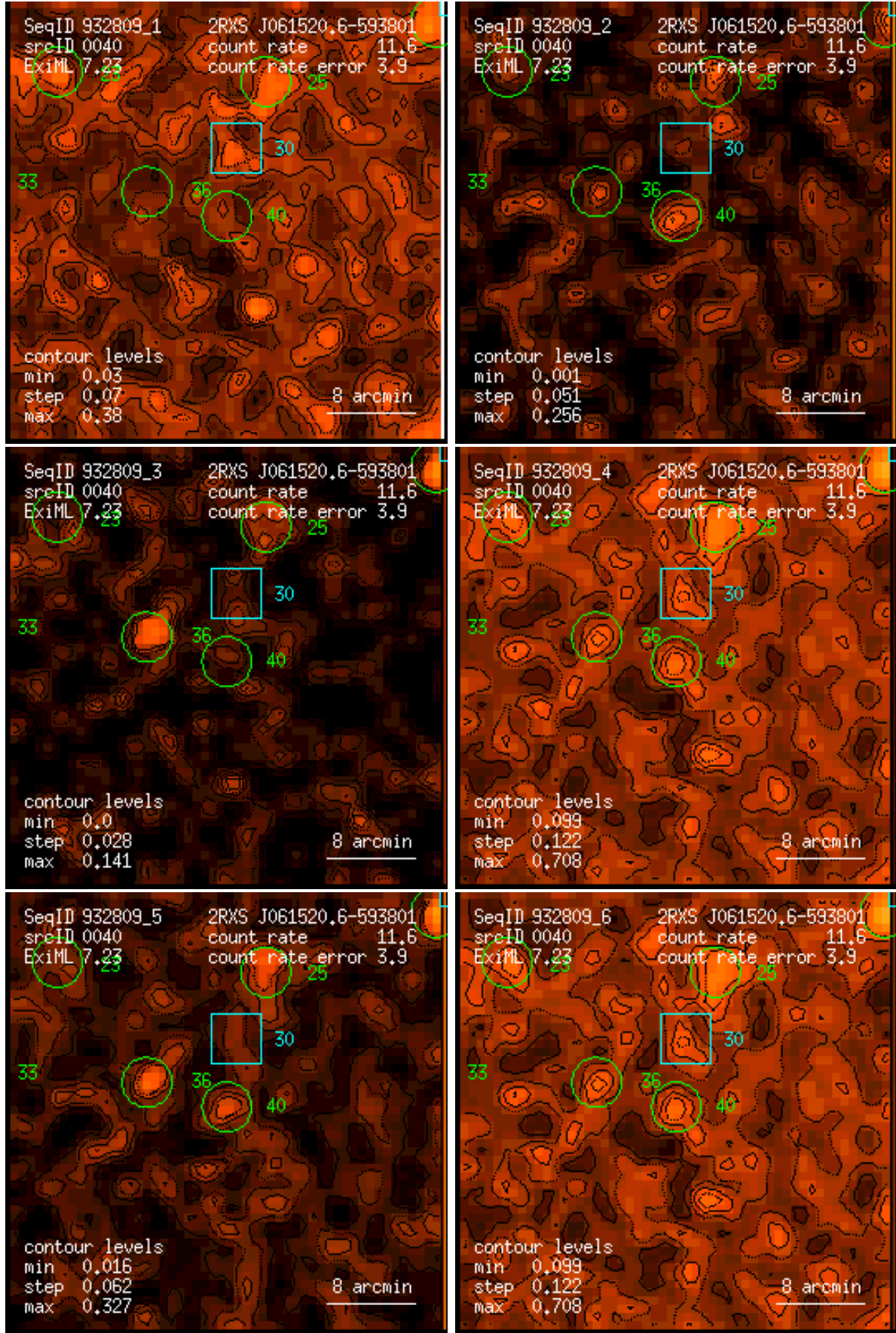
Figure 40: RASS 932809: detection 0040: band rate images, Gaussian filter: (1) PSPC channels 11 – 41, (2) 52 – 90, (3) 91 – 201, (4) 11 – 235, (5) 52 – 201, (6) 11 – 201. Broad band rates in counts/ks. Band rate contour levels in counts/ks/arcmin 2 .
