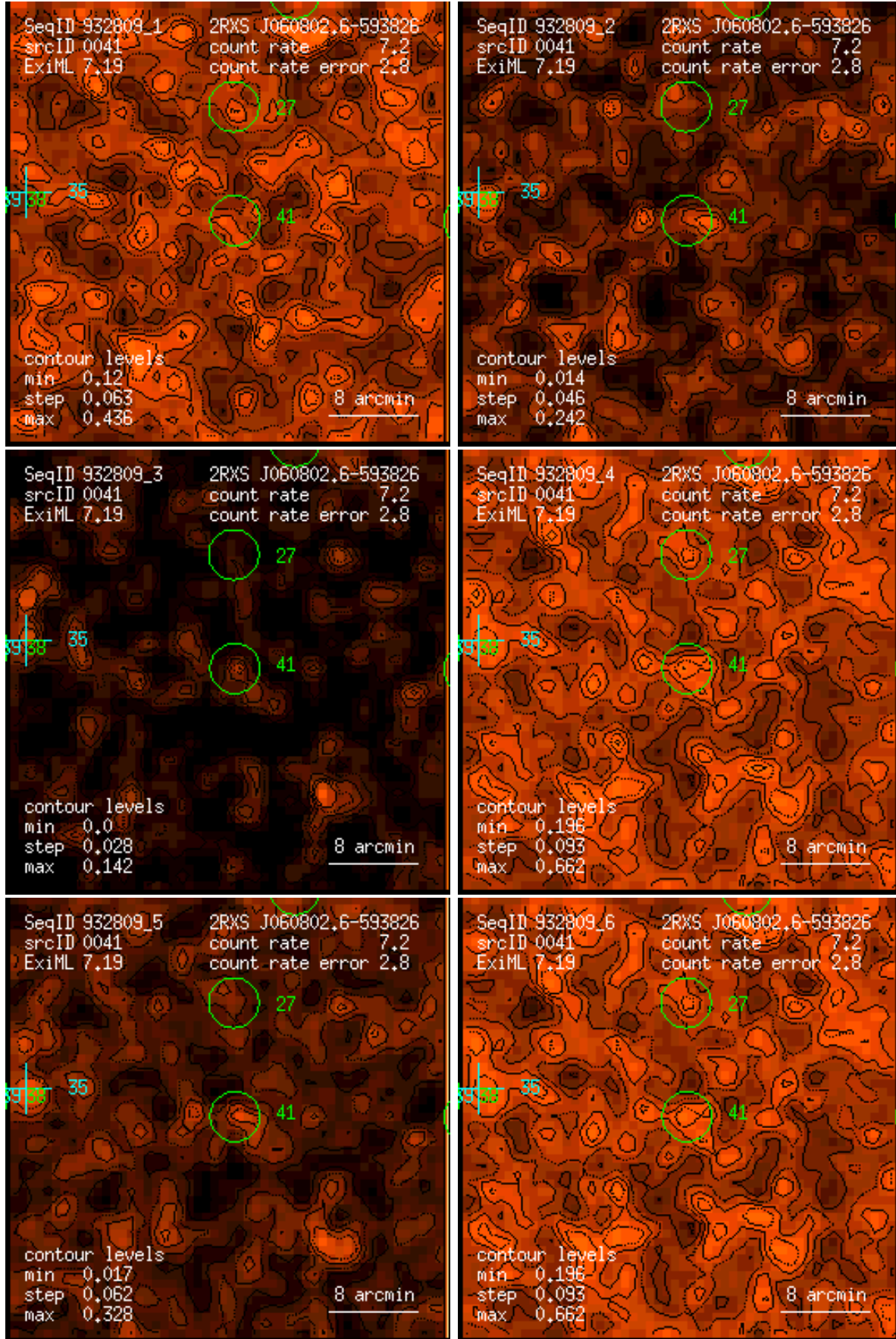
Figure 41: RASS 932809: detection 0041: band rate images, Gaussian filter: (1) PSPC channels 11 – 41, (2) 52 – 90, (3) 91 – 201, (4) 11 – 235, (5) 52 – 201, (6) 11 – 201. Broad band rates in counts/ks. Band rate contour levels in counts/ks/arcmin 2 .
