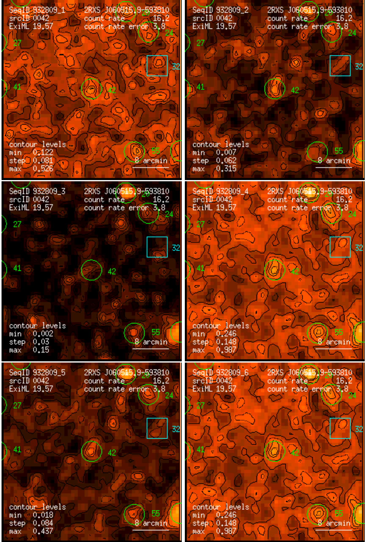
Figure 42: RASS 932809: detection 0042: band rate images, Gaussian filter: (1) PSPC channels 11 – 41, (2) 52 – 90, (3) 91 – 201, (4) 11 – 235, (5) 52 – 201, (6) 11 – 201. Broad band rates in counts/ks. Band rate contour levels in counts/ks/arcmin 2 .
