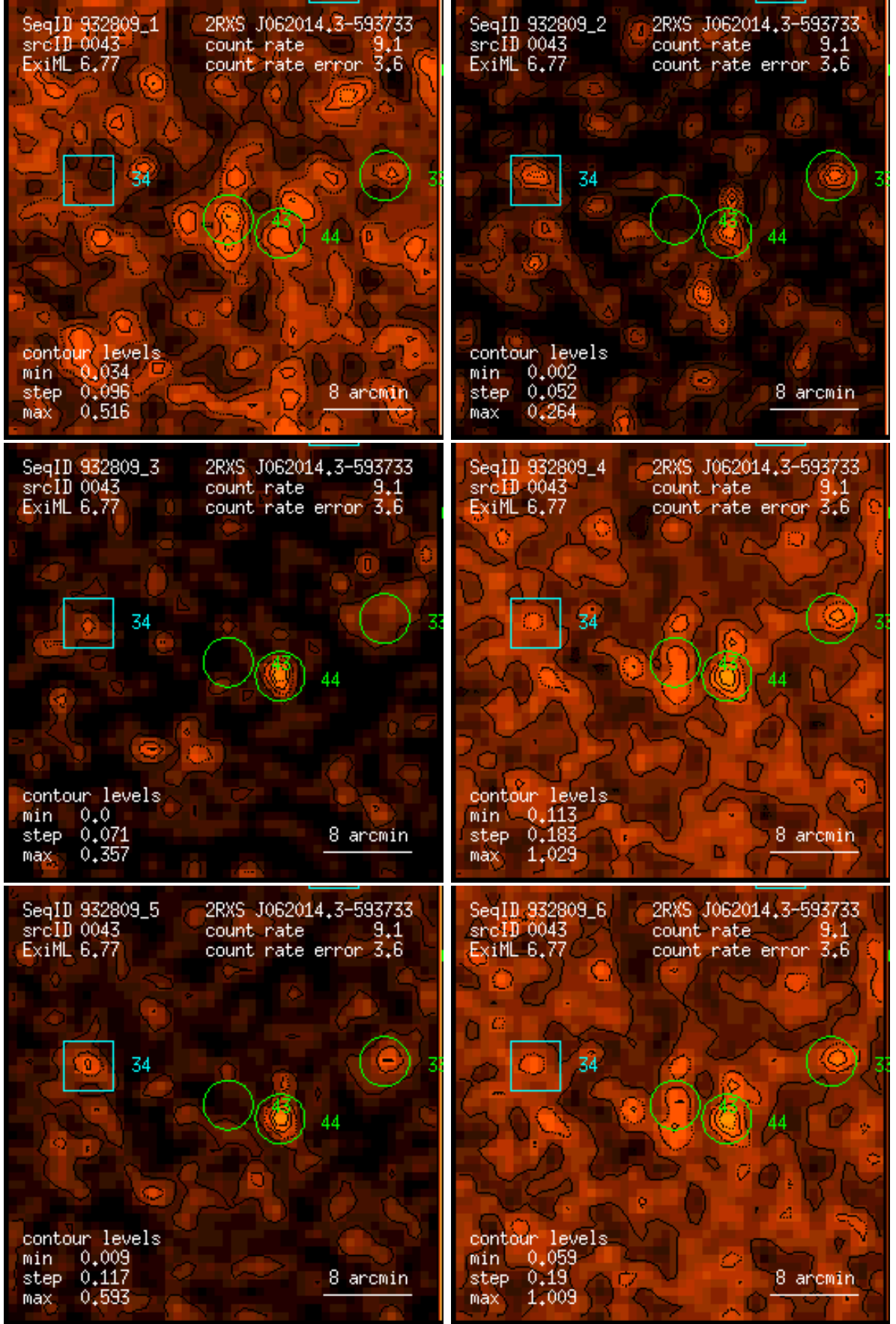
Figure 43: RASS 932809: detection 0043: band rate images, Gaussian filter: (1) PSPC channels 11 – 41, (2) 52 – 90, (3) 91 – 201, (4) 11 – 235, (5) 52 – 201, (6) 11 – 201. Broad band rates in counts/ks. Band rate contour levels in counts/ks/arcmin 2 .
