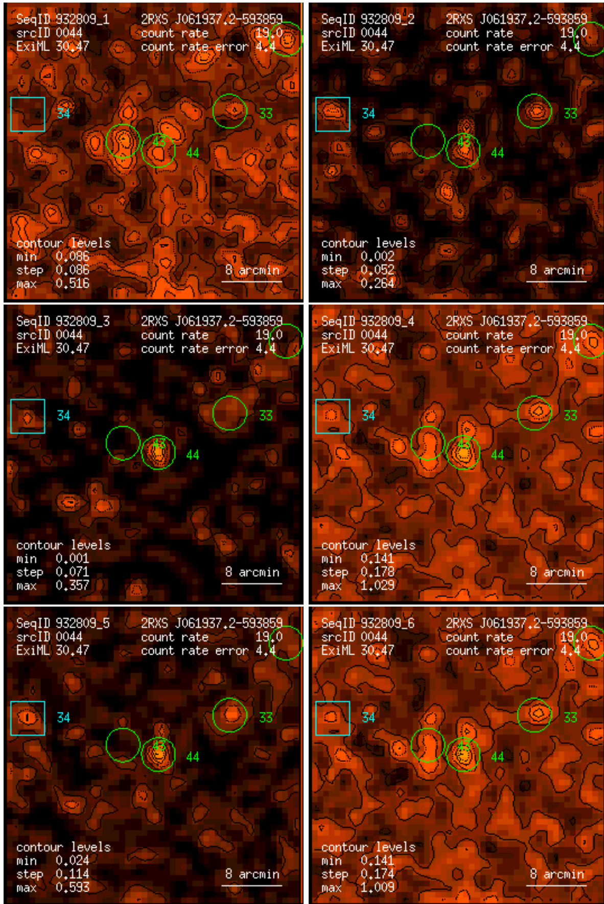
Figure 44: RASS 932809: detection 0044: band rate images, Gaussian filter: (1) PSPC channels 11 – 41, (2) 52 – 90, (3) 91 – 201, (4) 11 – 235, (5) 52 – 201, (6) 11 – 201. Broad band rates in counts/ks. Band rate contour levels in counts/ks/arcmin 2 .
