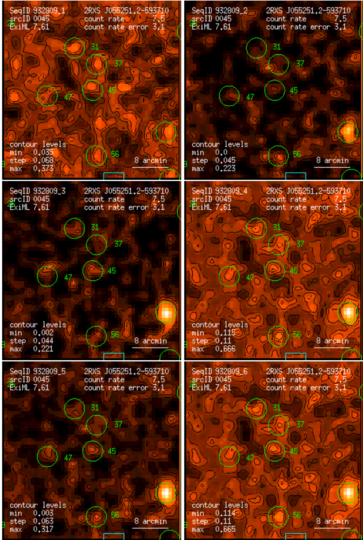
Figure 45: RASS 932809: detection 0045: band rate images, Gaussian filter: (1) PSPC channels 11 – 41, (2) 52 – 90, (3) 91 – 201, (4) 11 – 235, (5) 52 – 201, (6) 11 – 201. Broad band rates in counts/ks. Band rate contour levels in counts/ks/arcmin 2 .
