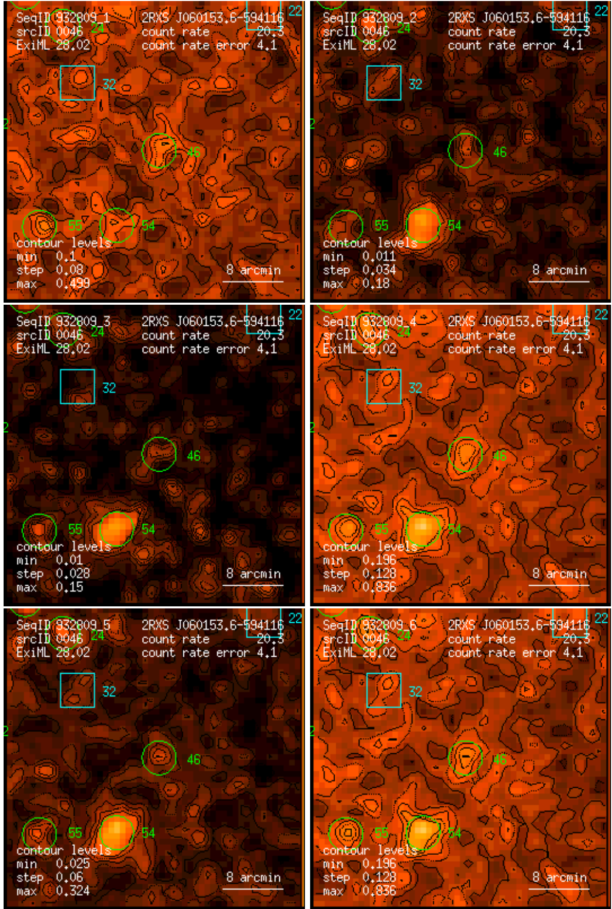
Figure 46: RASS 932809: detection 0046: band rate images, Gaussian filter: (1) PSPC channels 11 – 41, (2) 52 – 90, (3) 91 – 201, (4) 11 – 235, (5) 52 – 201, (6) 11 – 201. Broad band rates in counts/ks. Band rate contour levels in counts/ks/arcmin 2 .
