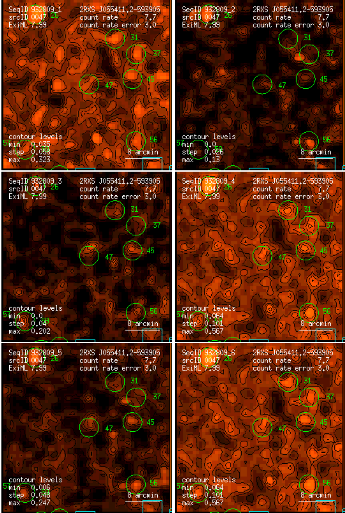
Figure 47: RASS 932809: detection 0047: band rate images, Gaussian filter: (1) PSPC channels 11 – 41, (2) 52 – 90, (3) 91 – 201, (4) 11 – 235, (5) 52 – 201, (6) 11 – 201. Broad band rates in counts/ks. Band rate contour levels in counts/ks/arcmin 2 .
