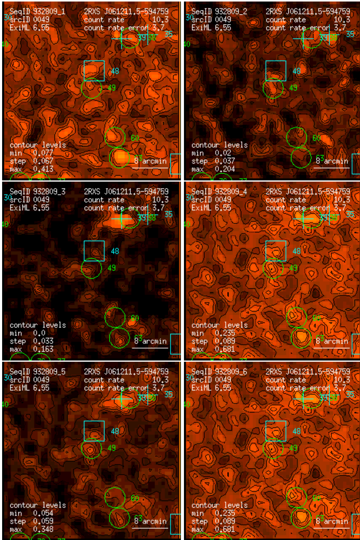
Figure 49: RASS 932809: detection 0049: band rate images, Gaussian filter: (1) PSPC channels 11 – 41, (2) 52 – 90, (3) 91 – 201, (4) 11 – 235, (5) 52 – 201, (6) 11 – 201. Broad band rates in counts/ks. Band rate contour levels in counts/ks/arcmin 2 .
