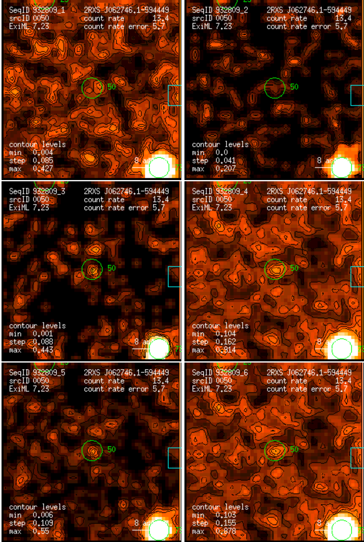
Figure 50: RASS 932809: detection 0050: band rate images, Gaussian filter: (1) PSPC channels 11 – 41, (2) 52 – 90, (3) 91 – 201, (4) 11 – 235, (5) 52 – 201, (6) 11 – 201. Broad band rates in counts/ks. Band rate contour levels in counts/ks/arcmin 2 .
