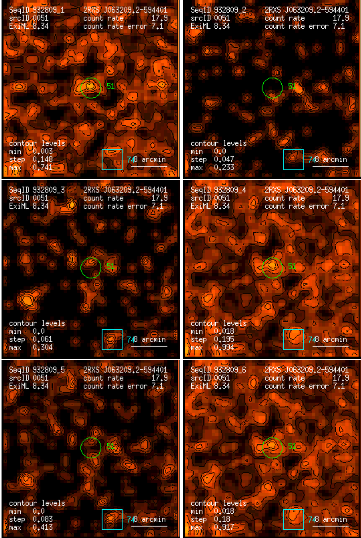
Figure 51: RASS 932809: detection 0051: band rate images, Gaussian filter: (1) PSPC channels 11 – 41, (2) 52 – 90, (3) 91 – 201, (4) 11 – 235, (5) 52 – 201, (6) 11 – 201. Broad band rates in counts/ks. Band rate contour levels in counts/ks/arcmin 2 .
