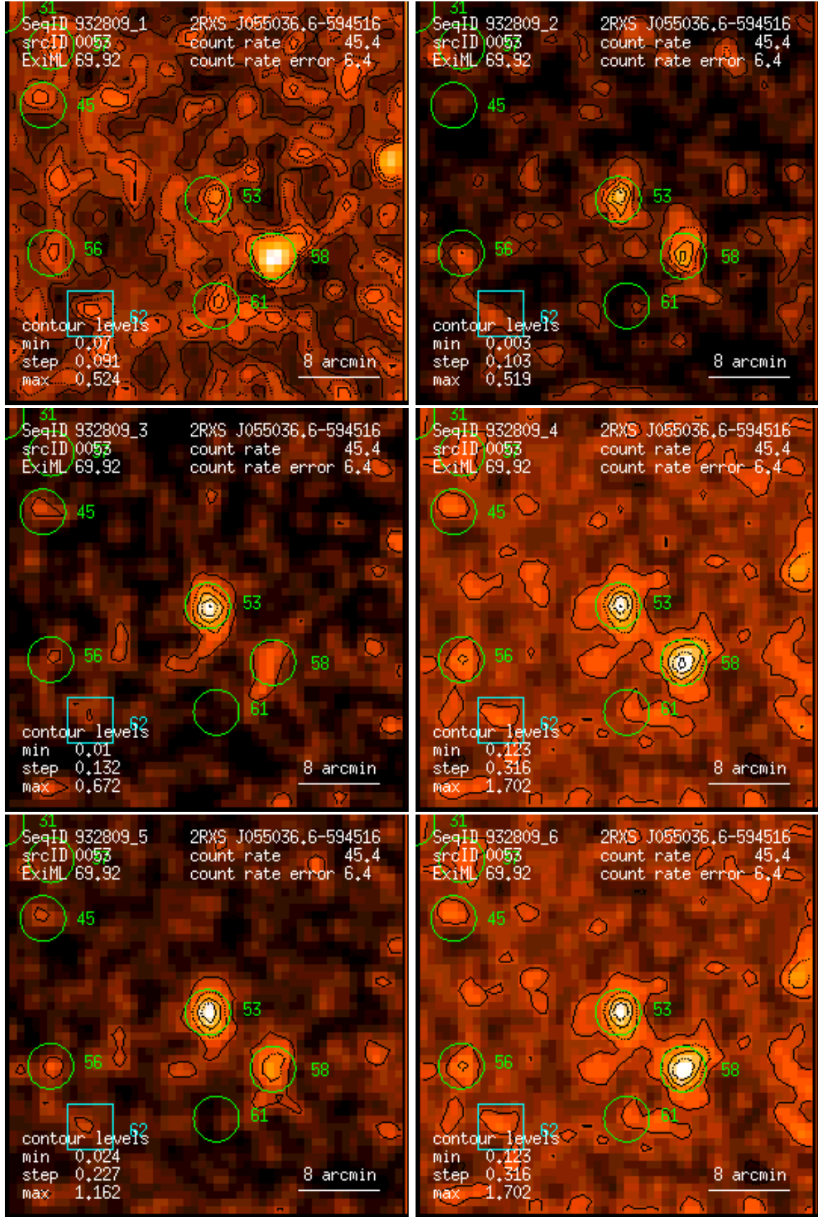
Figure 53: RASS 932809: detection 0053: band rate images, Gaussian filter: (1) PSPC channels 11 – 41, (2) 52 – 90, (3) 91 – 201, (4) 11 – 235, (5) 52 – 201, (6) 11 – 201. Broad band rates in counts/ks. Band rate contour levels in counts/ks/arcmin 2 .
