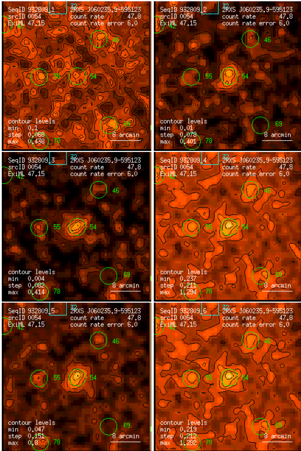
Figure 54: RASS 932809: detection 0054: band rate images, Gaussian filter: (1) PSPC channels 11 – 41, (2) 52 – 90, (3) 91 – 201, (4) 11 – 235, (5) 52 – 201, (6) 11 – 201. Broad band rates in counts/ks. Band rate contour levels in counts/ks/arcmin 2 .
