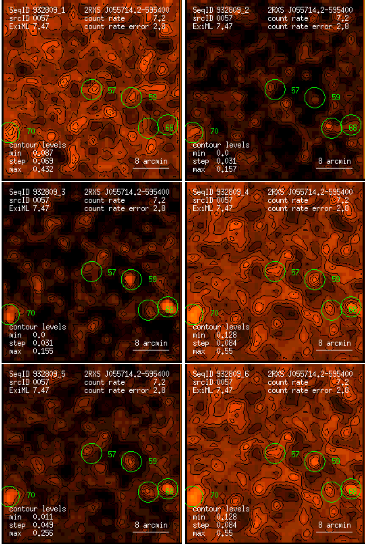
Figure 57: RASS 932809: detection 0057: band rate images, Gaussian filter: (1) PSPC channels 11 – 41, (2) 52 – 90, (3) 91 – 201, (4) 11 – 235, (5) 52 – 201, (6) 11 – 201. Broad band rates in counts/ks. Band rate contour levels in counts/ks/arcmin 2 .
