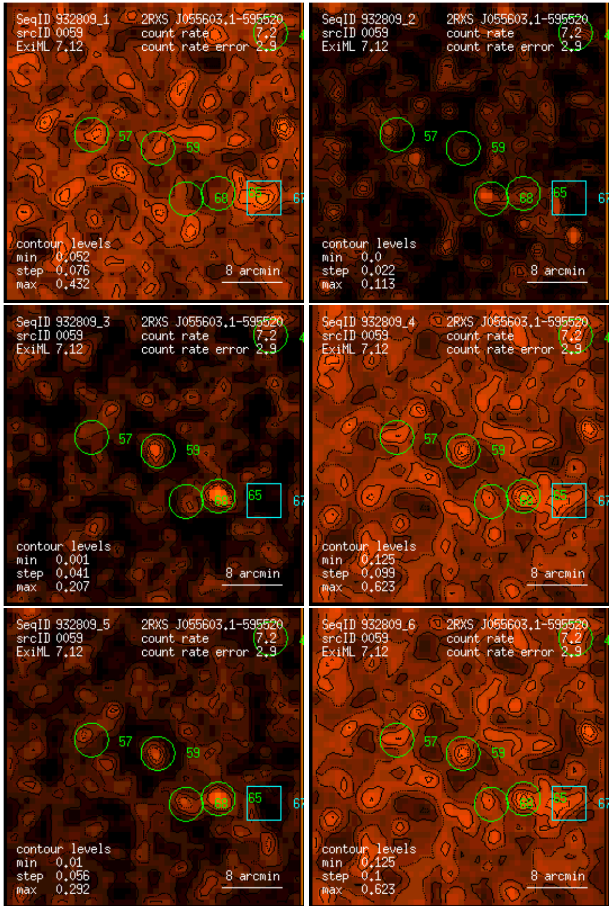
Figure 59: RASS 932809: detection 0059: band rate images, Gaussian filter: (1) PSPC channels 11 – 41, (2) 52 – 90, (3) 91 – 201, (4) 11 – 235, (5) 52 – 201, (6) 11 – 201. Broad band rates in counts/ks. Band rate contour levels in counts/ks/arcmin 2 .
