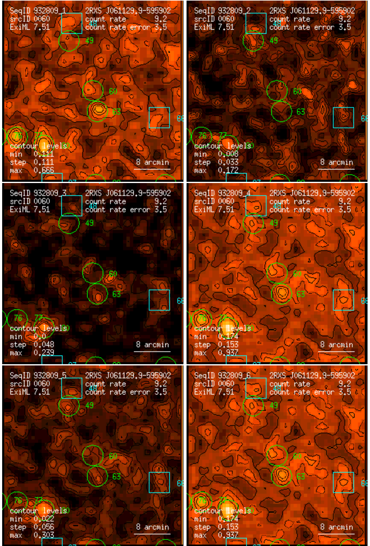
Figure 60: RASS 932809: detection 0060: band rate images, Gaussian filter: (1) PSPC channels 11 – 41, (2) 52 – 90, (3) 91 – 201, (4) 11 – 235, (5) 52 – 201, (6) 11 – 201. Broad band rates in counts/ks. Band rate contour levels in counts/ks/arcmin 2 .
