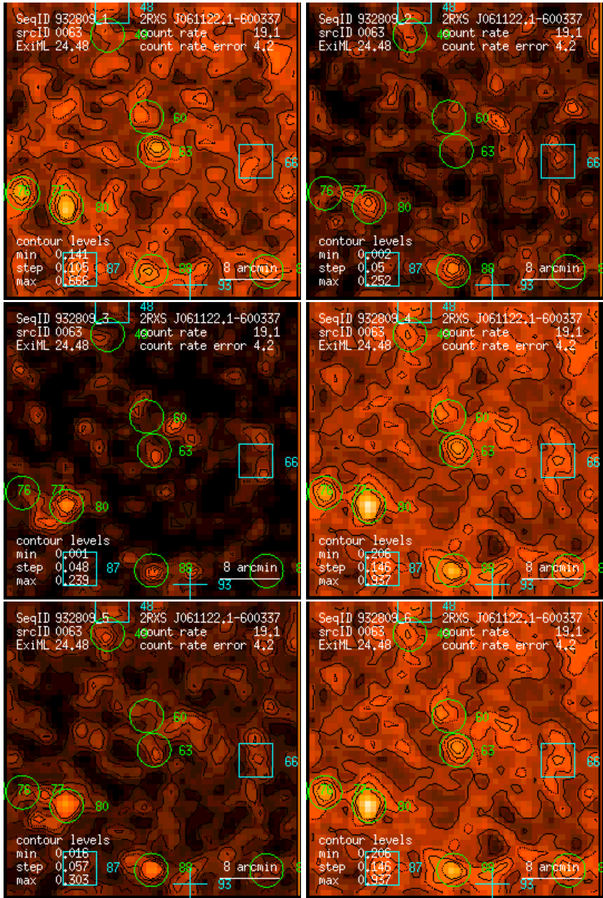
Figure 63: RASS 932809: detection 0063: band rate images, Gaussian filter: (1) PSPC channels 11 – 41, (2) 52 – 90, (3) 91 – 201, (4) 11 – 235, (5) 52 – 201, (6) 11 – 201. Broad band rates in counts/ks. Band rate contour levels in counts/ks/arcmin 2 .
