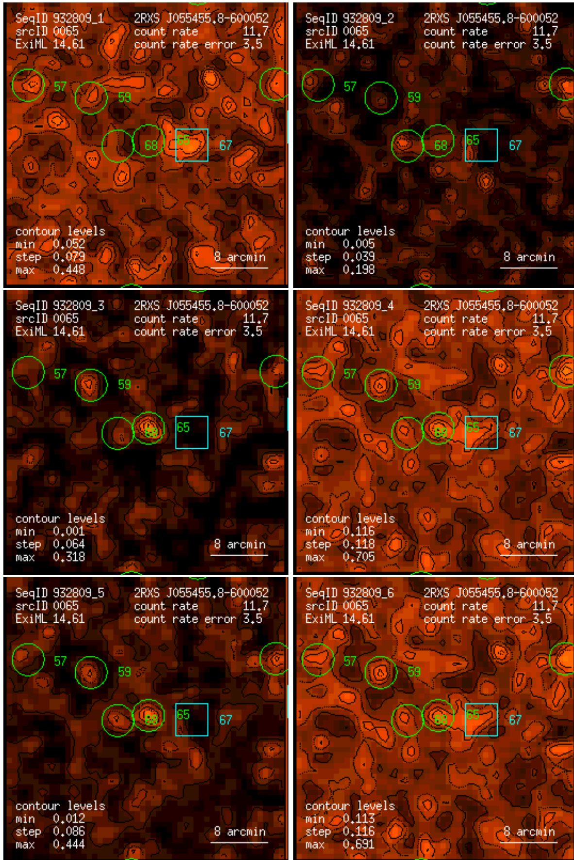
Figure 65: RASS 932809: detection 0065: band rate images, Gaussian filter: (1) PSPC channels 11 – 41, (2) 52 – 90, (3) 91 – 201, (4) 11 – 235, (5) 52 – 201, (6) 11 – 201. Broad band rates in counts/ks. Band rate contour levels in counts/ks/arcmin 2 .
