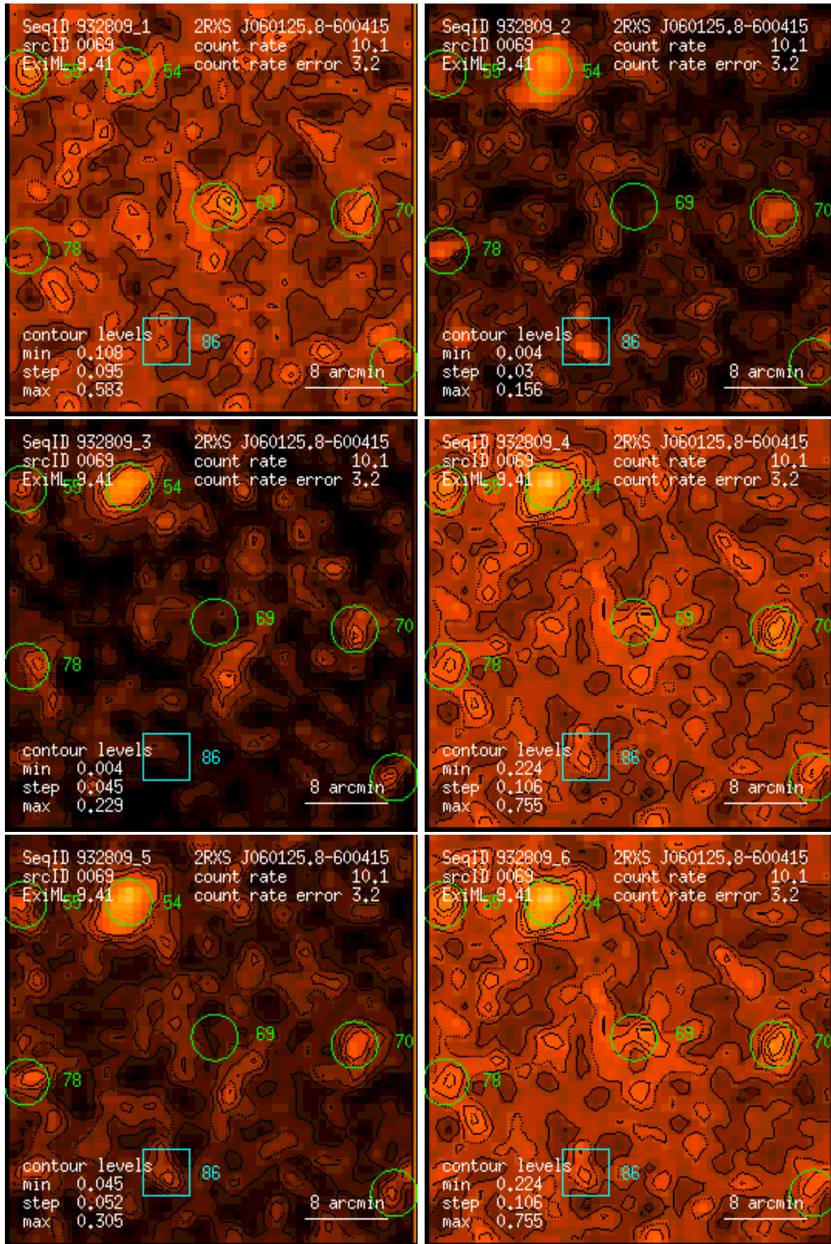
Figure 69: RASS 932809: detection 0069: band rate images, Gaussian filter: (1) PSPC channels 11 – 41, (2) 52 – 90, (3) 91 – 201, (4) 11 – 235, (5) 52 – 201, (6) 11 – 201. Broad band rates in counts/ks. Band rate contour levels in counts/ks/arcmin 2 .
