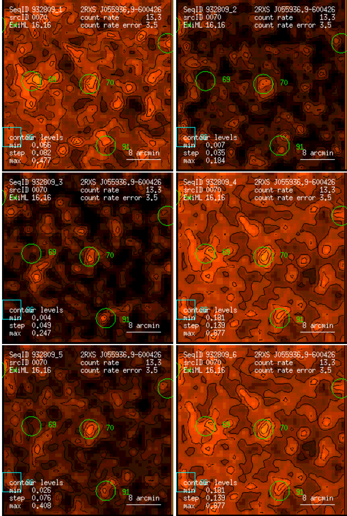
Figure 70: RASS 932809: detection 0070: band rate images, Gaussian filter: (1) PSPC channels 11 – 41, (2) 52 – 90, (3) 91 – 201, (4) 11 – 235, (5) 52 – 201, (6) 11 – 201. Broad band rates in counts/ks. Band rate contour levels in counts/ks/arcmin 2 .
