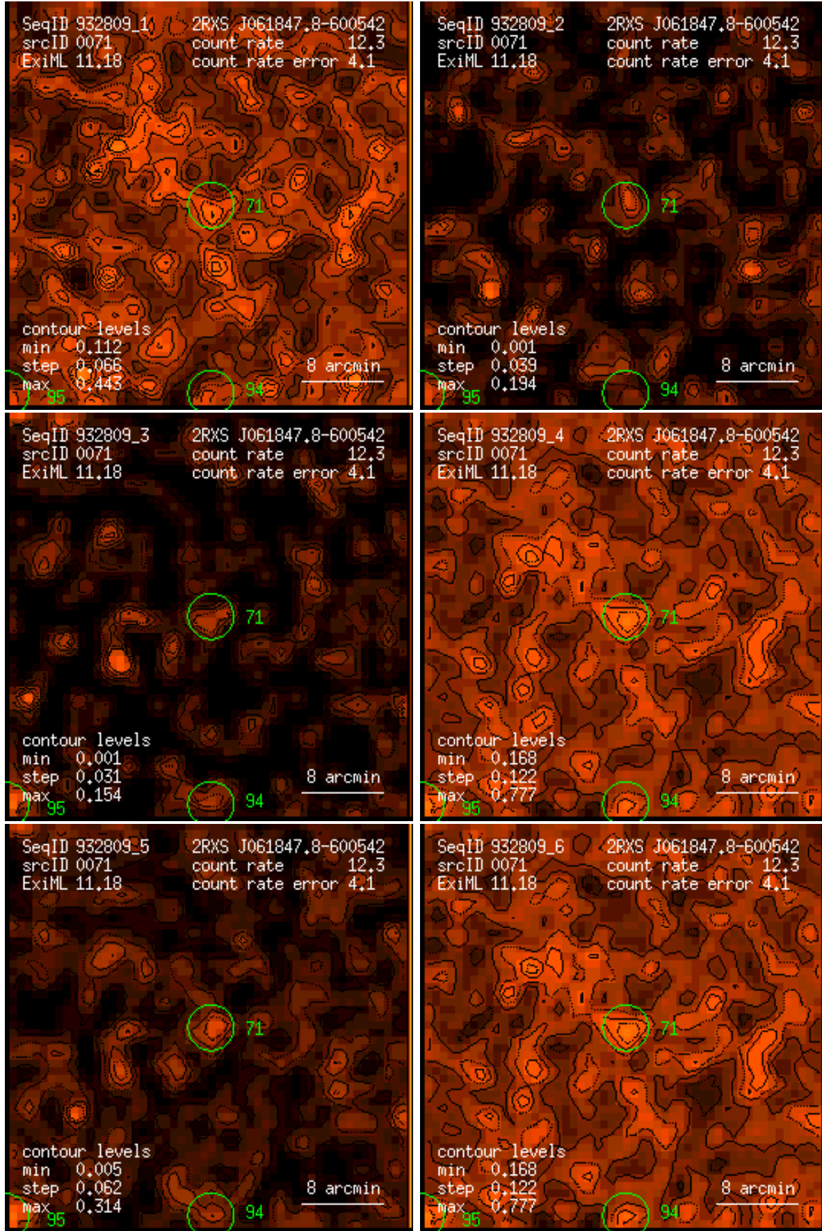
Figure 71: RASS 932809: detection 0071: band rate images, Gaussian filter: (1) PSPC channels 11 – 41, (2) 52 – 90, (3) 91 – 201, (4) 11 – 235, (5) 52 – 201, (6) 11 – 201. Broad band rates in counts/ks. Band rate contour levels in counts/ks/arcmin 2 .
