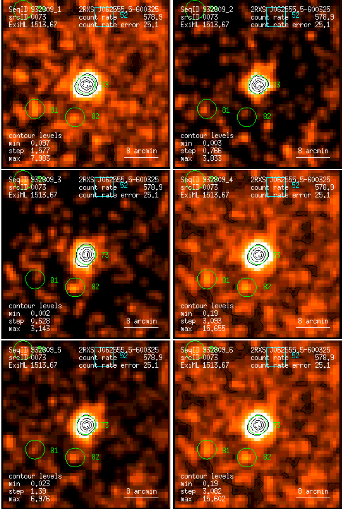
Figure 73: RASS 932809: detection 0073: band rate images, Gaussian filter: (1) PSPC channels 11 – 41, (2) 52 – 90, (3) 91 – 201, (4) 11 – 235, (5) 52 – 201, (6) 11 – 201. Broad band rates in counts/ks. Band rate contour levels in counts/ks/arcmin 2 .
