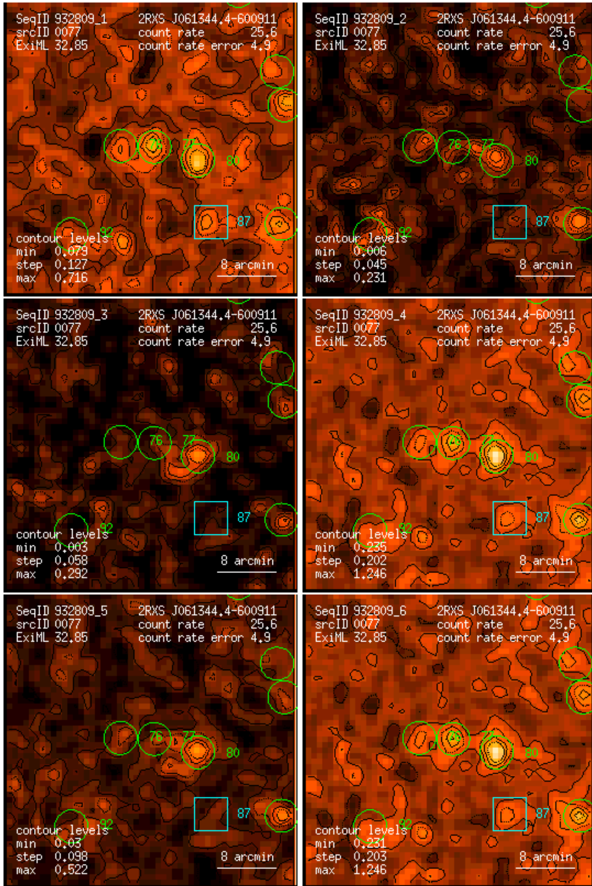
Figure 77: RASS 932809: detection 0077: band rate images, Gaussian filter: (1) PSPC channels 11 – 41, (2) 52 – 90, (3) 91 – 201, (4) 11 – 235, (5) 52 – 201, (6) 11 – 201. Broad band rates in counts/ks. Band rate contour levels in counts/ks/arcmin 2 .
