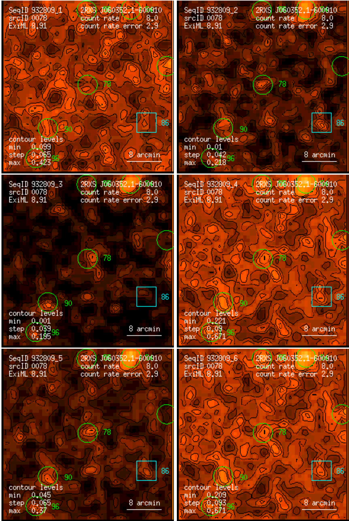
Figure 78: RASS 932809: detection 0078: band rate images, Gaussian filter: (1) PSPC channels 11 – 41, (2) 52 – 90, (3) 91 – 201, (4) 11 – 235, (5) 52 – 201, (6) 11 – 201. Broad band rates in counts/ks. Band rate contour levels in counts/ks/arcmin 2 .
