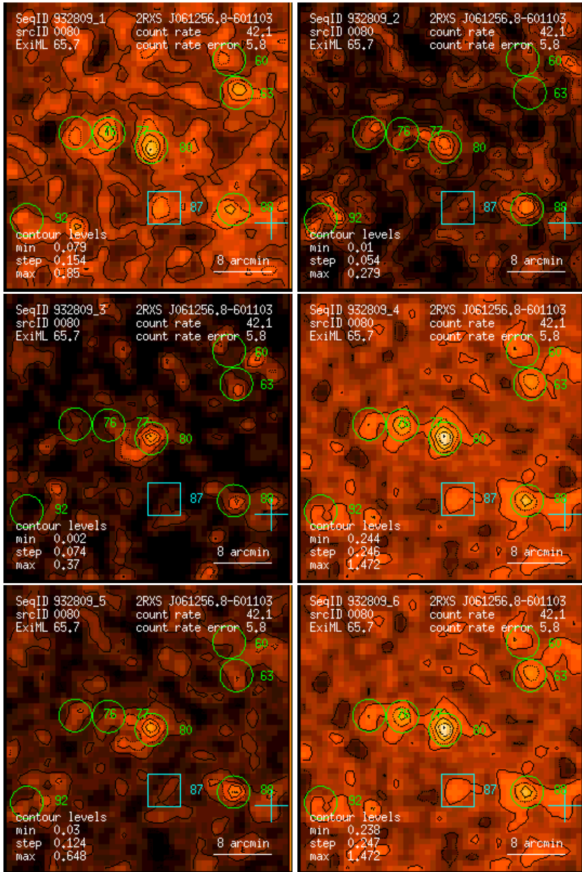
Figure 80: RASS 932809: detection 0080: band rate images, Gaussian filter: (1) PSPC channels 11 – 41, (2) 52 – 90, (3) 91 – 201, (4) 11 – 235, (5) 52 – 201, (6) 11 – 201. Broad band rates in counts/ks. Band rate contour levels in counts/ks/arcmin 2 .
