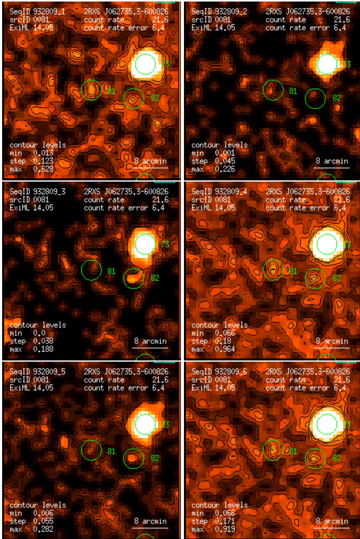
Figure 81: RASS 932809: detection 0081: band rate images, Gaussian filter: (1) PSPC channels 11 – 41, (2) 52 – 90, (3) 91 – 201, (4) 11 – 235, (5) 52 – 201, (6) 11 – 201. Broad band rates in counts/ks. Band rate contour levels in counts/ks/arcmin 2 .
