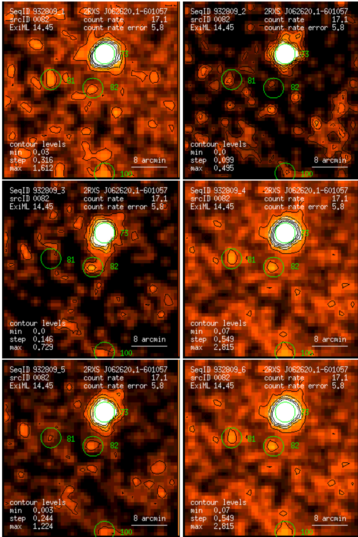
Figure 82: RASS 932809: detection 0082: band rate images, Gaussian filter: (1) PSPC channels 11 – 41, (2) 52 – 90, (3) 91 – 201, (4) 11 – 235, (5) 52 – 201, (6) 11 – 201. Broad band rates in counts/ks. Band rate contour levels in counts/ks/arcmin 2 .
