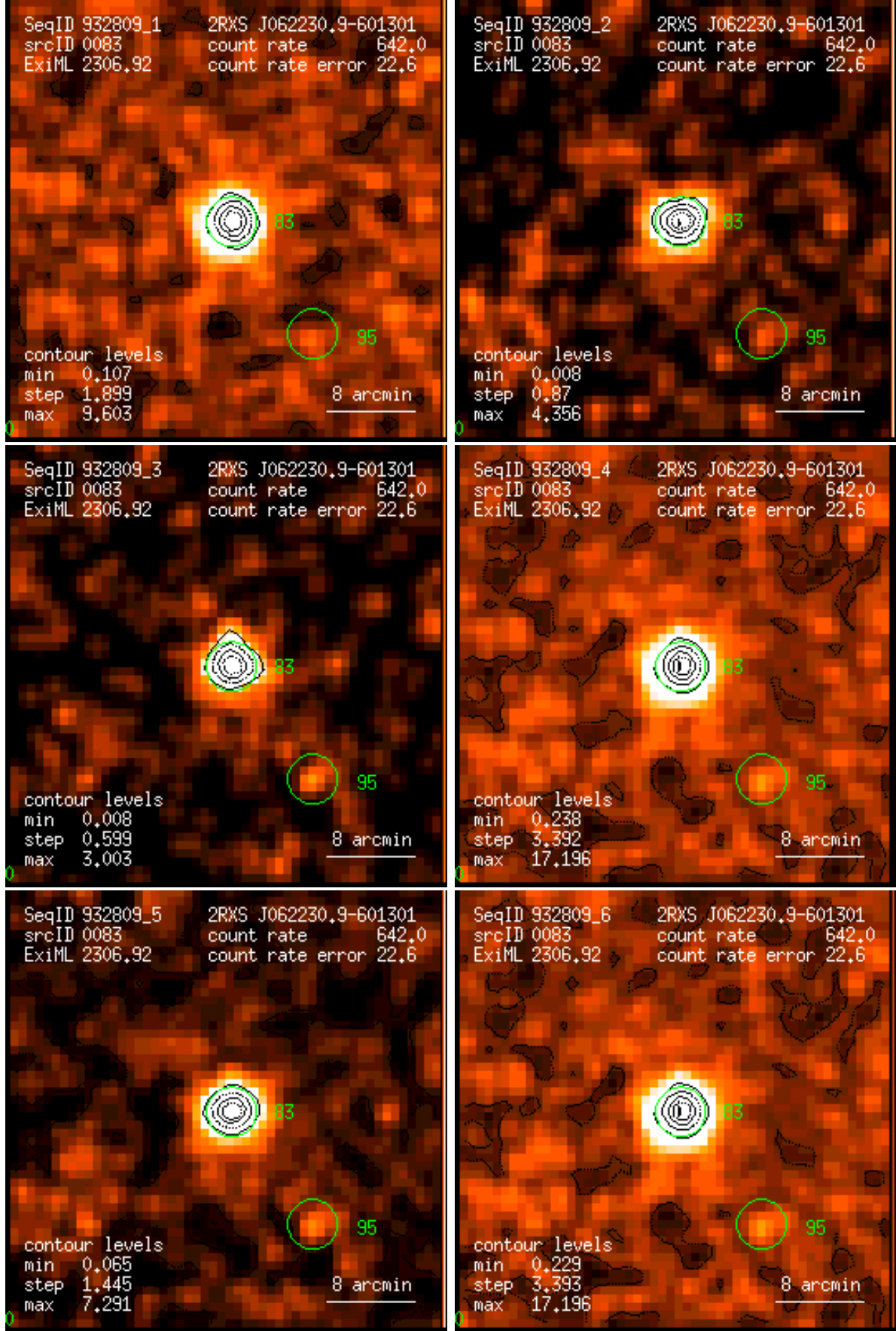
Figure 83: RASS 932809: detection 0083: band rate images, Gaussian filter: (1) PSPC channels 11 – 41, (2) 52 – 90, (3) 91 – 201, (4) 11 – 235, (5) 52 – 201, (6) 11 – 201. Broad band rates in counts/ks. Band rate contour levels in counts/ks/arcmin 2 .
