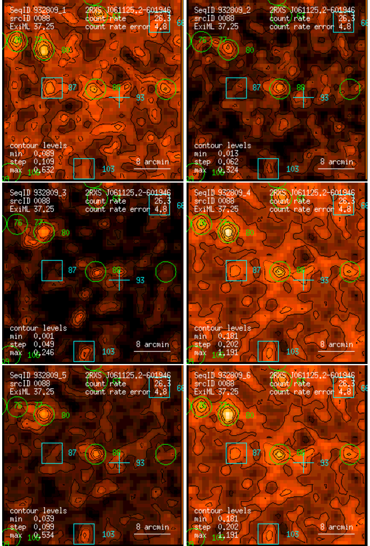
Figure 88: RASS 932809: detection 0088: band rate images, Gaussian filter: (1) PSPC channels 11 – 41, (2) 52 – 90, (3) 91 – 201, (4) 11 – 235, (5) 52 – 201, (6) 11 – 201. Broad band rates in counts/ks. Band rate contour levels in counts/ks/arcmin 2 .
