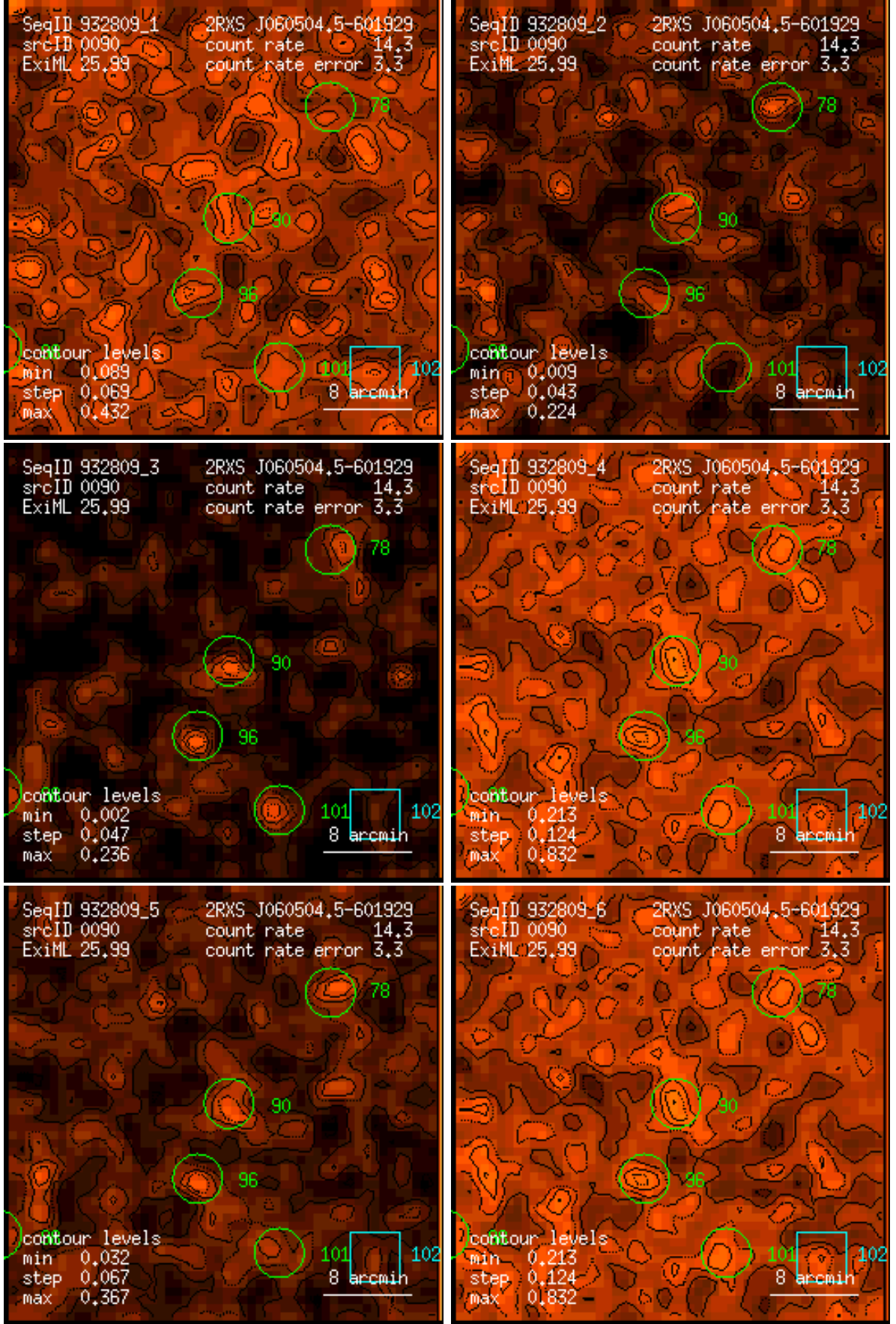
Figure 90: RASS 932809: detection 0090: band rate images, Gaussian filter: (1) PSPC channels 11 – 41, (2) 52 – 90, (3) 91 – 201, (4) 11 – 235, (5) 52 – 201, (6) 11 – 201. Broad band rates in counts/ks. Band rate contour levels in counts/ks/arcmin 2 .
