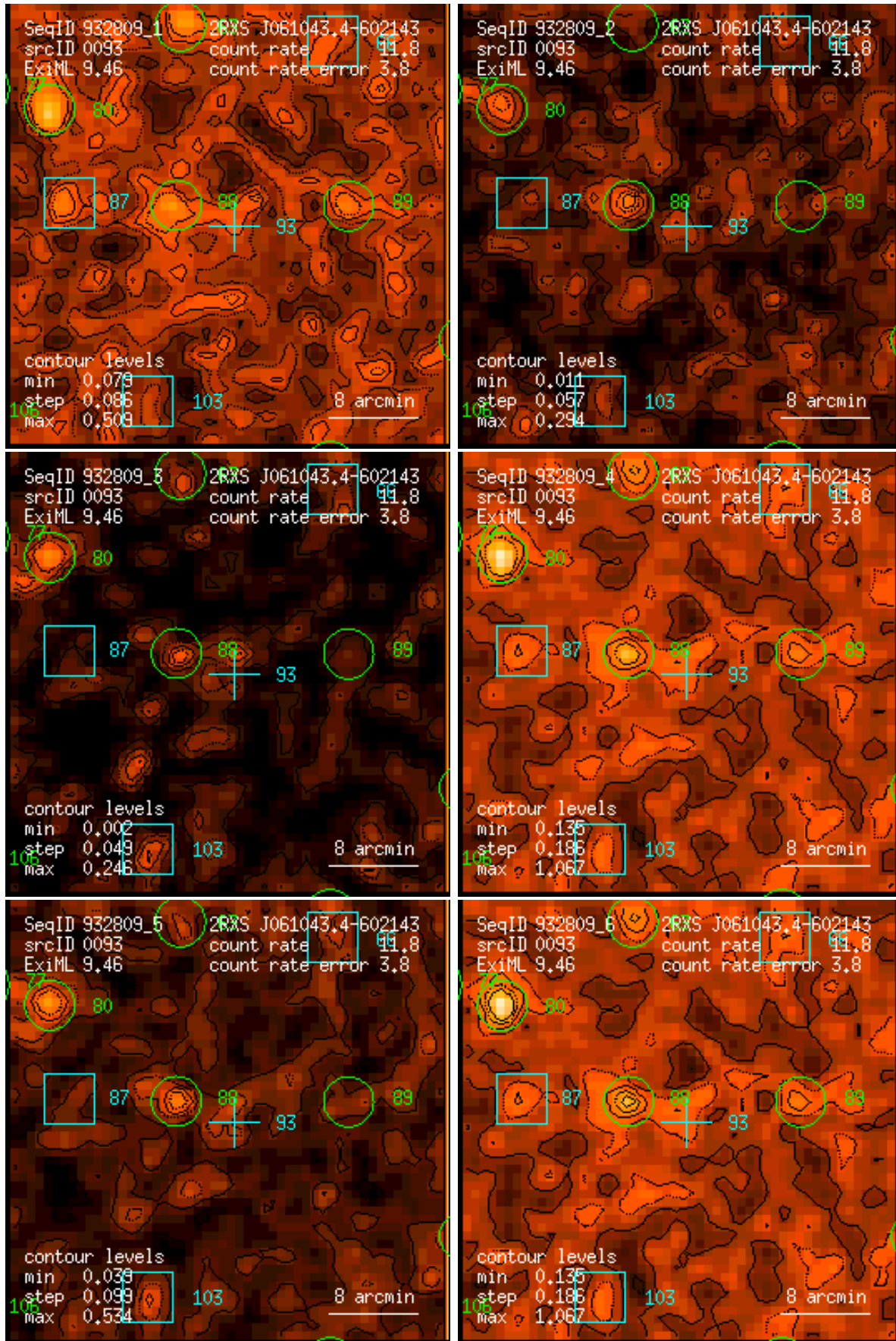
Figure 93: RASS 932809: detection 0093: band rate images, Gaussian filter: (1) PSPC channels 11 – 41, (2) 52 – 90, (3) 91 – 201, (4) 11 – 235, (5) 52 – 201, (6) 11 – 201. Broad band rates in counts/ks. Band rate contour levels in counts/ks/arcmin 2 .
