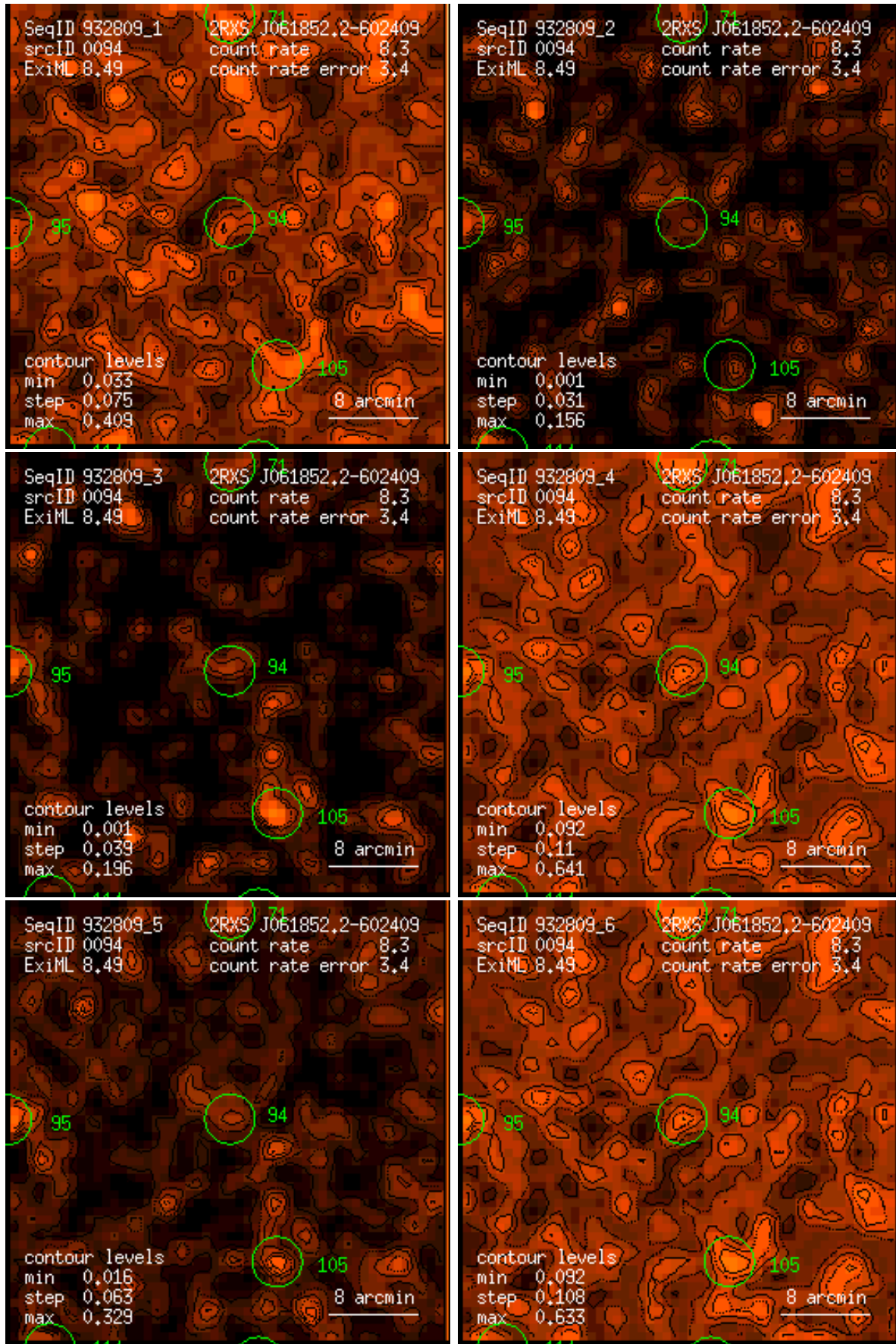
Figure 94: RASS 932809: detection 0094: band rate images, Gaussian filter: (1) PSPC channels 11 – 41, (2) 52 – 90, (3) 91 – 201, (4) 11 – 235, (5) 52 – 201, (6) 11 – 201. Broad band rates in counts/ks. Band rate contour levels in counts/ks/arcmin 2 .
