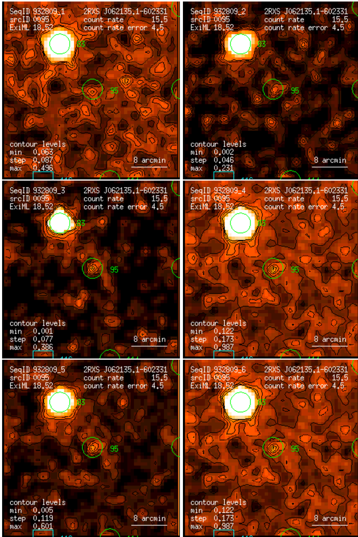
Figure 95: RASS 932809: detection 0095: band rate images, Gaussian filter: (1) PSPC channels 11 – 41, (2) 52 – 90, (3) 91 – 201, (4) 11 – 235, (5) 52 – 201, (6) 11 – 201. Broad band rates in counts/ks. Band rate contour levels in counts/ks/arcmin 2 .
