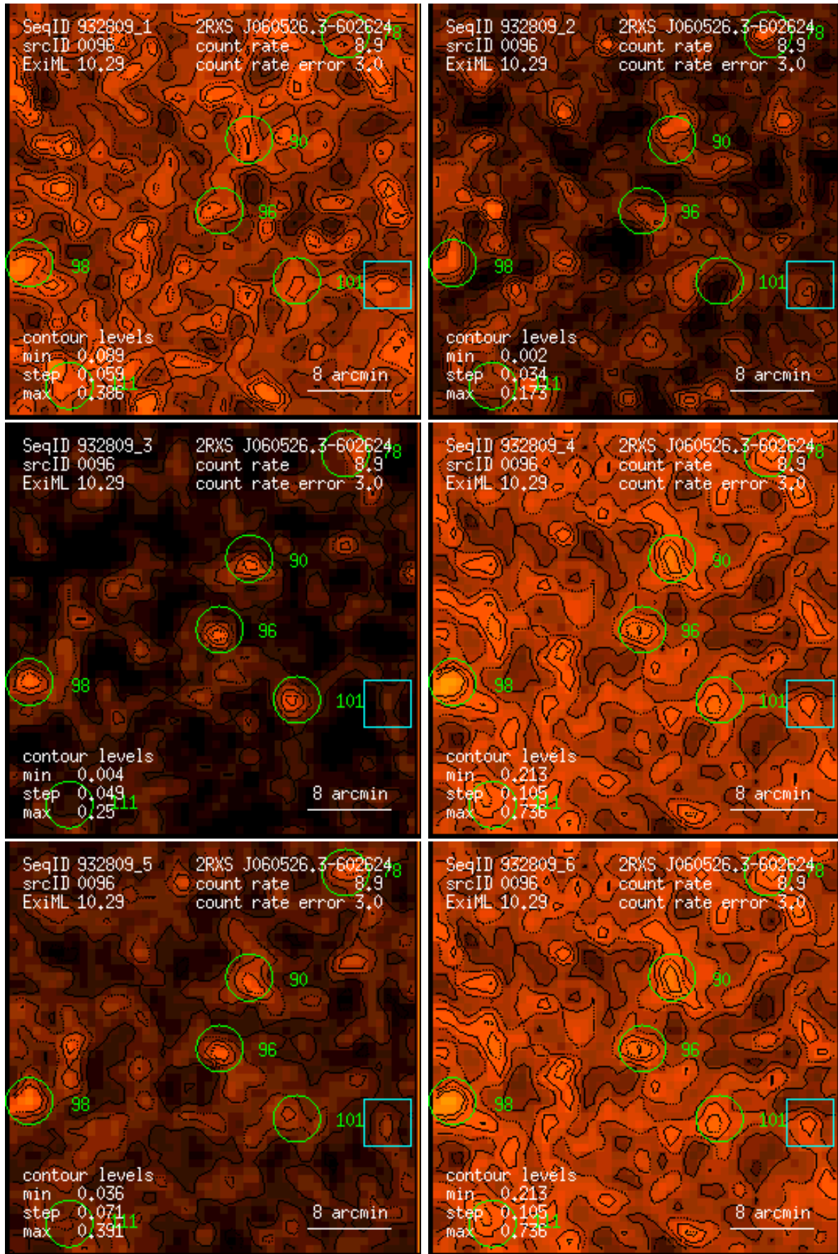
Figure 96: RASS 932809: detection 0096: band rate images, Gaussian filter: (1) PSPC channels 11 – 41, (2) 52 – 90, (3) 91 – 201, (4) 11 – 235, (5) 52 – 201, (6) 11 – 201. Broad band rates in counts/ks. Band rate contour levels in counts/ks/arcmin 2 .
