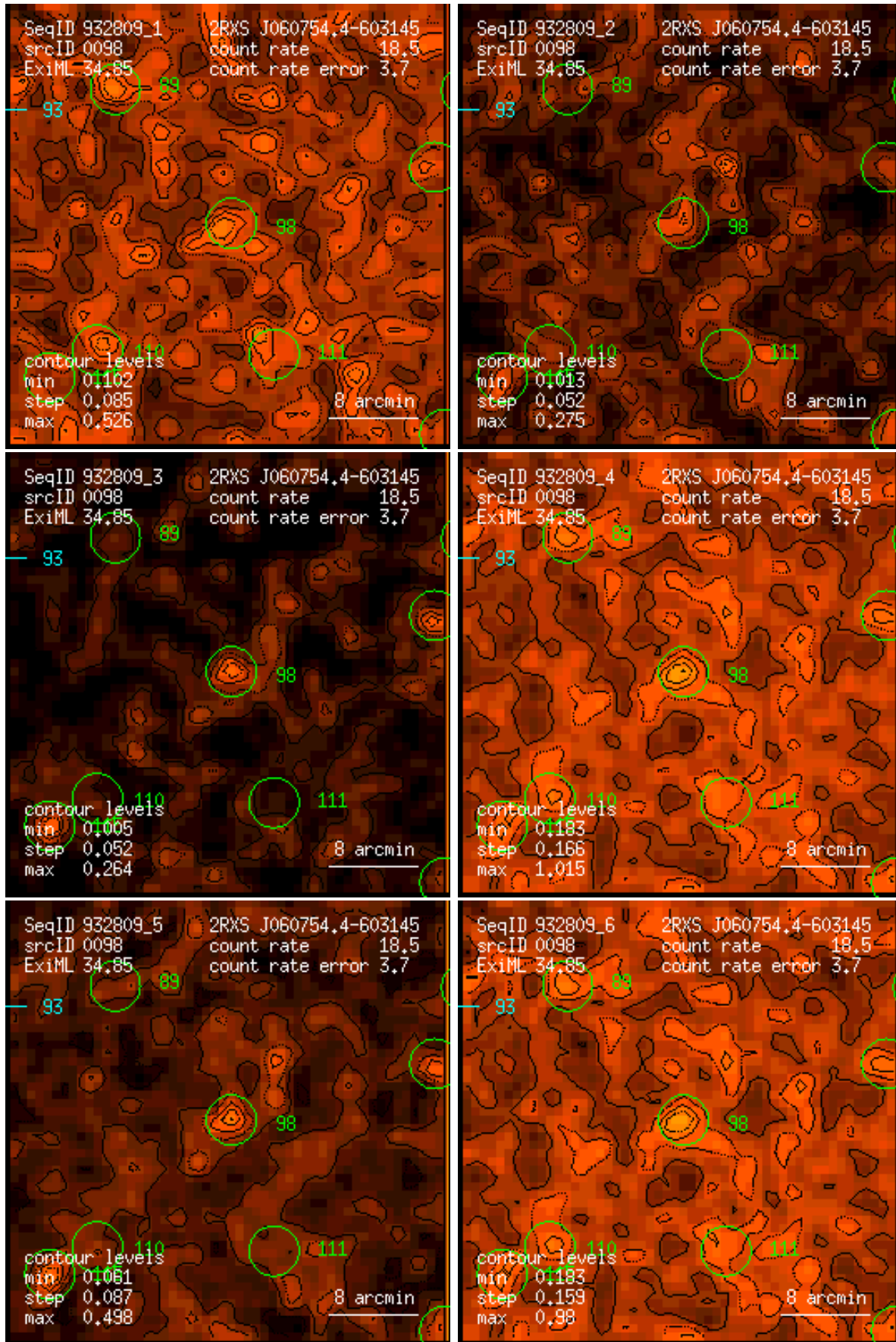
Figure 98: RASS 932809: detection 0098: band rate images, Gaussian filter: (1) PSPC channels 11 – 41, (2) 52 – 90, (3) 91 – 201, (4) 11 – 235, (5) 52 – 201, (6) 11 – 201. Broad band rates in counts/ks. Band rate contour levels in counts/ks/arcmin 2 .
