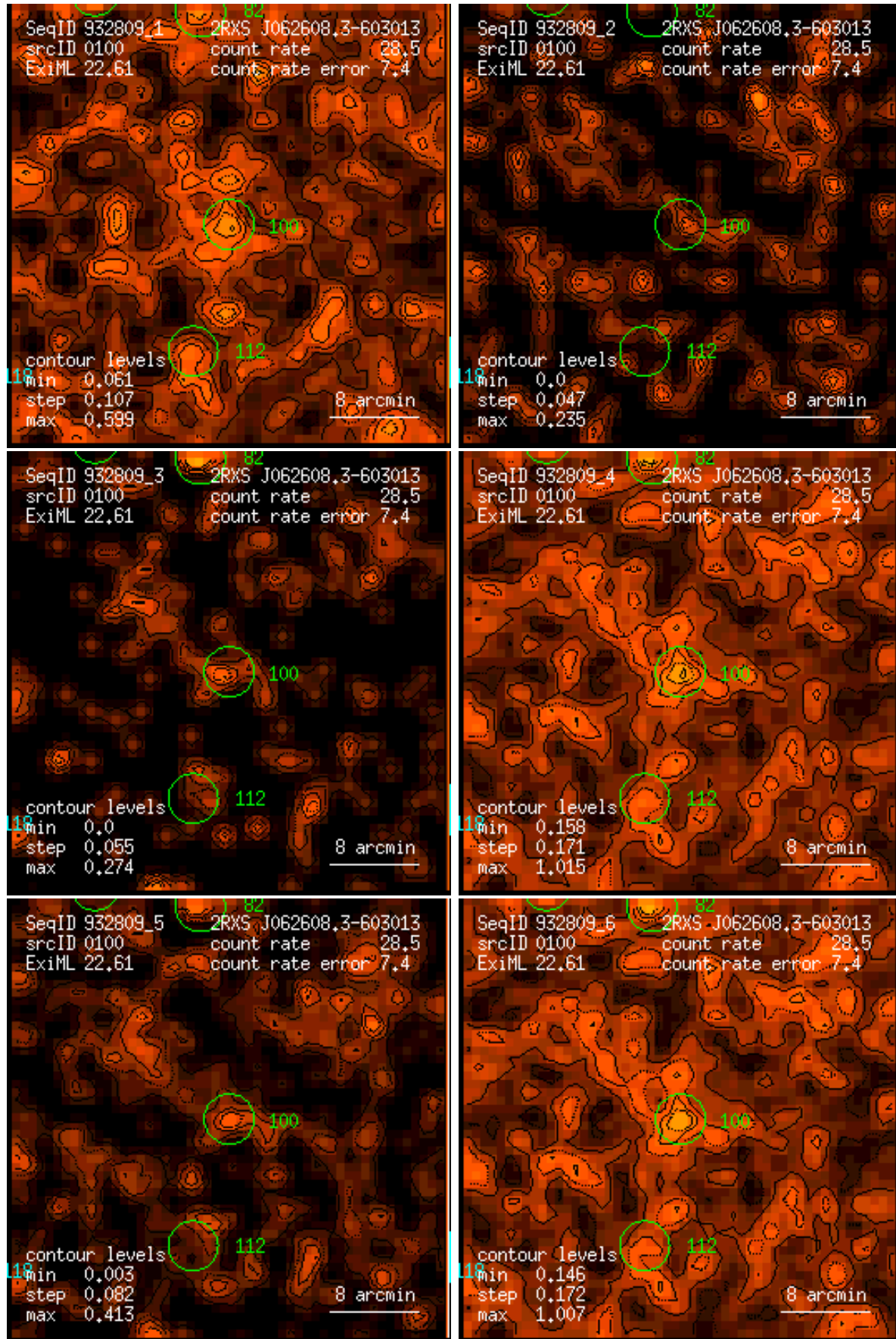
Figure 100: RASS 932809: detection 0100: band rate images, Gaussian filter: (1) PSPC channels 11 – 41, (2) 52 – 90, (3) 91 – 201, (4) 11 – 235, (5) 52 – 201, (6) 11 – 201. Broad band rates in counts/ks. Band rate contour levels in counts/ks/arcmin 2 .
