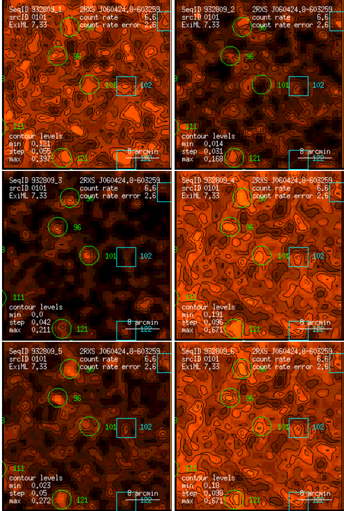
Figure 101: RASS 932809: detection 0101: band rate images, Gaussian filter: (1) PSPC channels 11 – 41, (2) 52 – 90, (3) 91 – 201, (4) 11 – 235, (5) 52 – 201, (6) 11 – 201. Broad band rates in counts/ks. Band rate contour levels in counts/ks/arcmin 2 .
