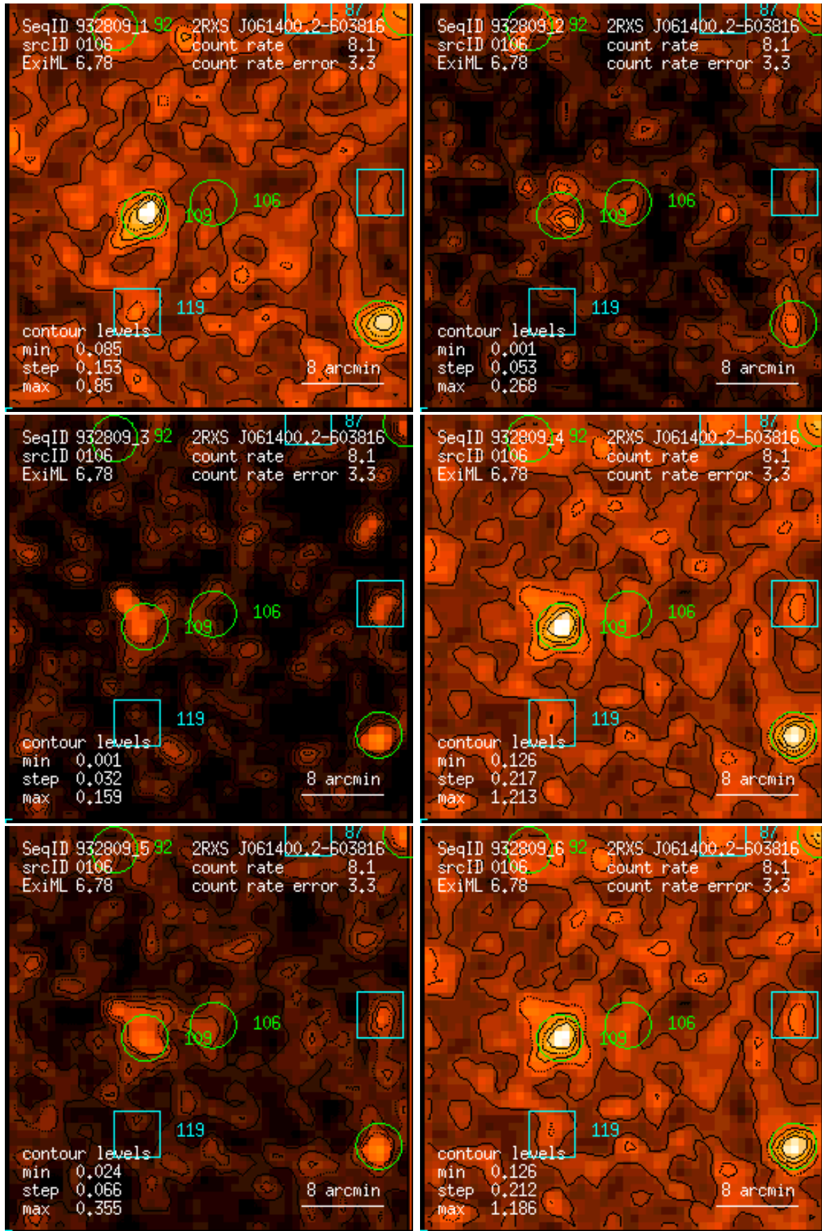
Figure 106: RASS 932809: detection 0106: band rate images, Gaussian filter: (1) PSPC channels 11 – 41, (2) 52 – 90, (3) 91 – 201, (4) 11 – 235, (5) 52 – 201, (6) 11 – 201. Broad band rates in counts/ks. Band rate contour levels in counts/ks/arcmin 2 .
