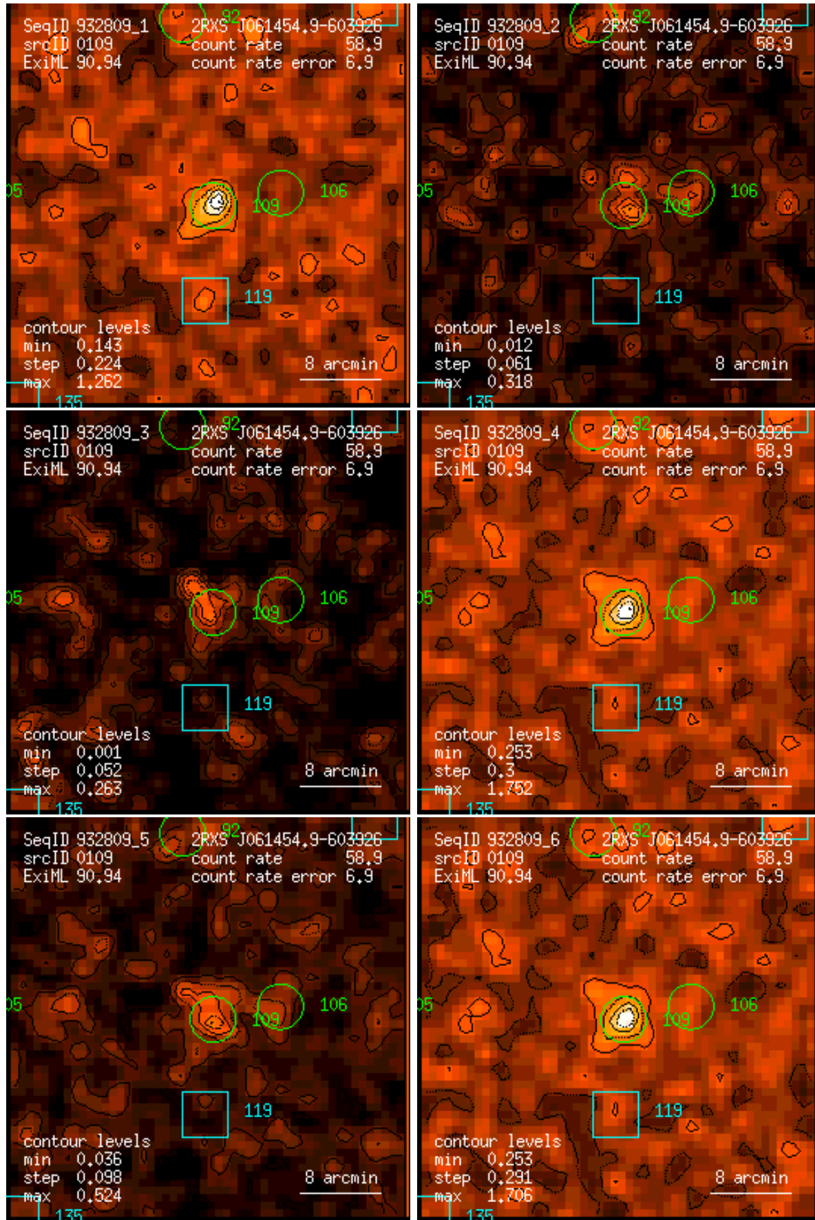
Figure 109: RASS 932809: detection 0109: band rate images, Gaussian filter: (1) PSPC channels 11 – 41, (2) 52 – 90, (3) 91 – 201, (4) 11 – 235, (5) 52 – 201, (6) 11 – 201. Broad band rates in counts/ks. Band rate contour levels in counts/ks/arcmin 2 .
