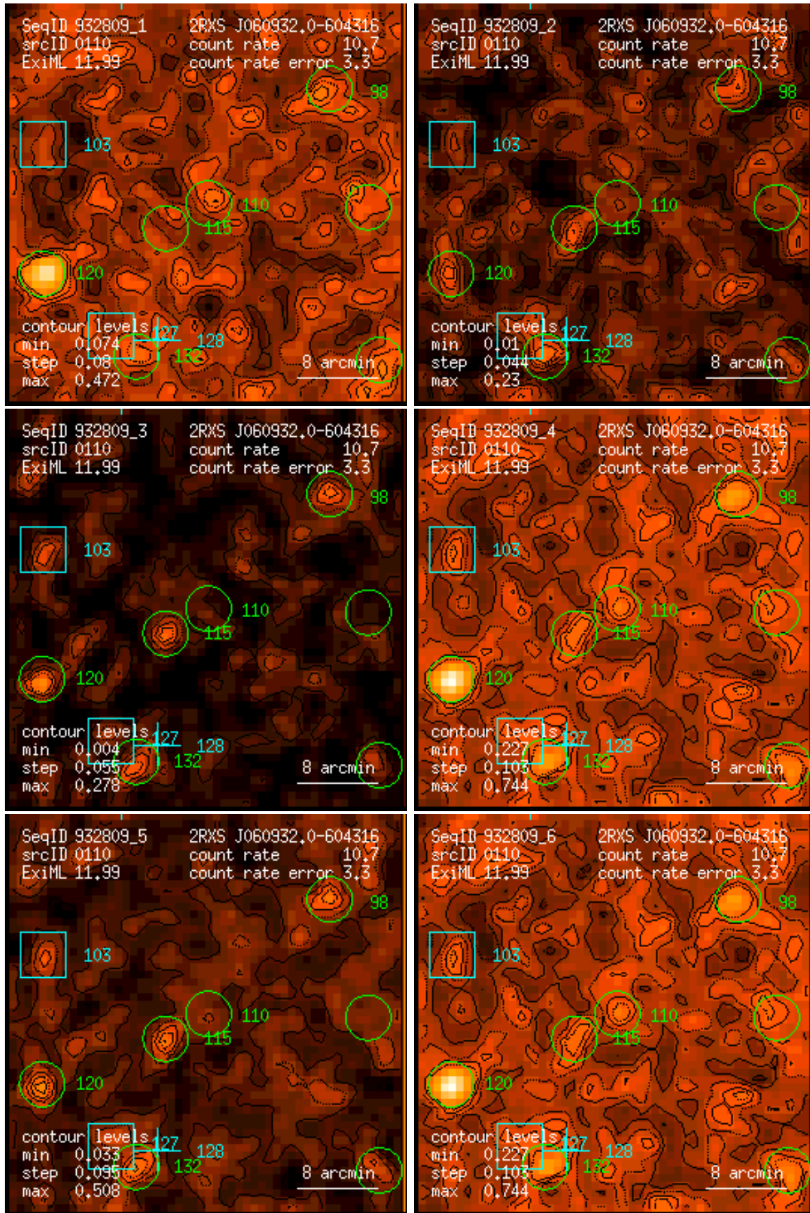
Figure 110: RASS 932809: detection 0110: band rate images, Gaussian filter: (1) PSPC channels 11 – 41, (2) 52 – 90, (3) 91 – 201, (4) 11 – 235, (5) 52 – 201, (6) 11 – 201. Broad band rates in counts/ks. Band rate contour levels in counts/ks/arcmin 2 .
