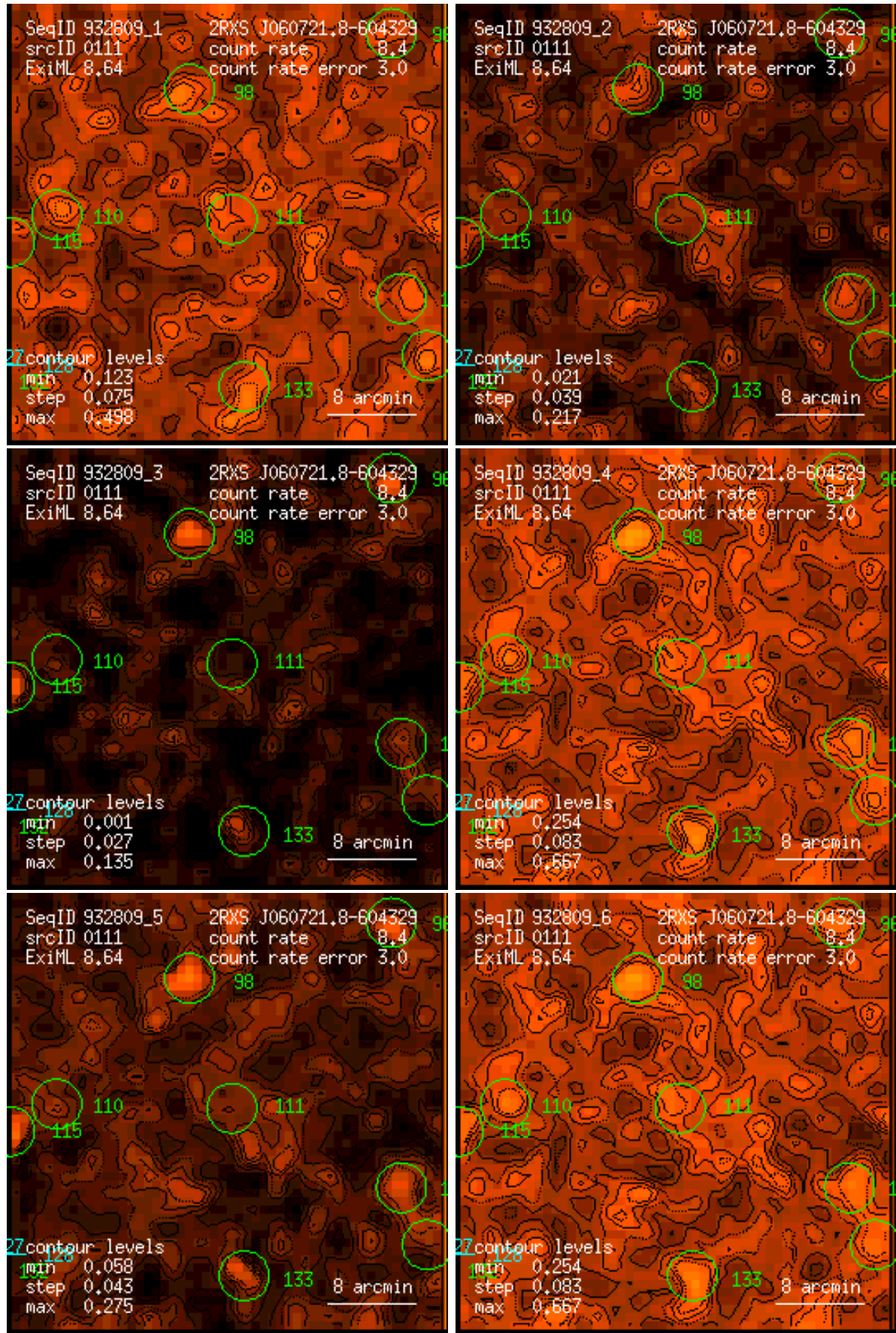
Figure 111: RASS 932809: detection 0111: band rate images, Gaussian filter: (1) PSPC channels 11 – 41, (2) 52 – 90, (3) 91 – 201, (4) 11 – 235, (5) 52 – 201, (6) 11 – 201. Broad band rates in counts/ks. Band rate contour levels in counts/ks/arcmin 2 .
