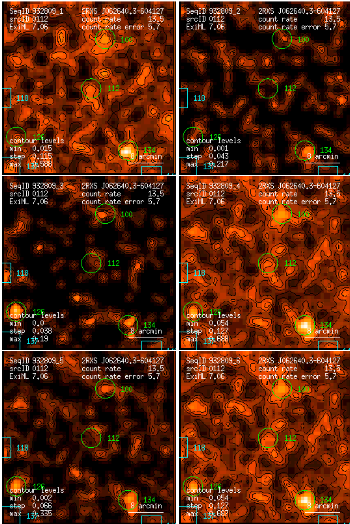
Figure 112: RASS 932809: detection 0112: band rate images, Gaussian filter: (1) PSPC channels 11 – 41, (2) 52 – 90, (3) 91 – 201, (4) 11 – 235, (5) 52 – 201, (6) 11 – 201. Broad band rates in counts/ks. Band rate contour levels in counts/ks/arcmin 2 .
