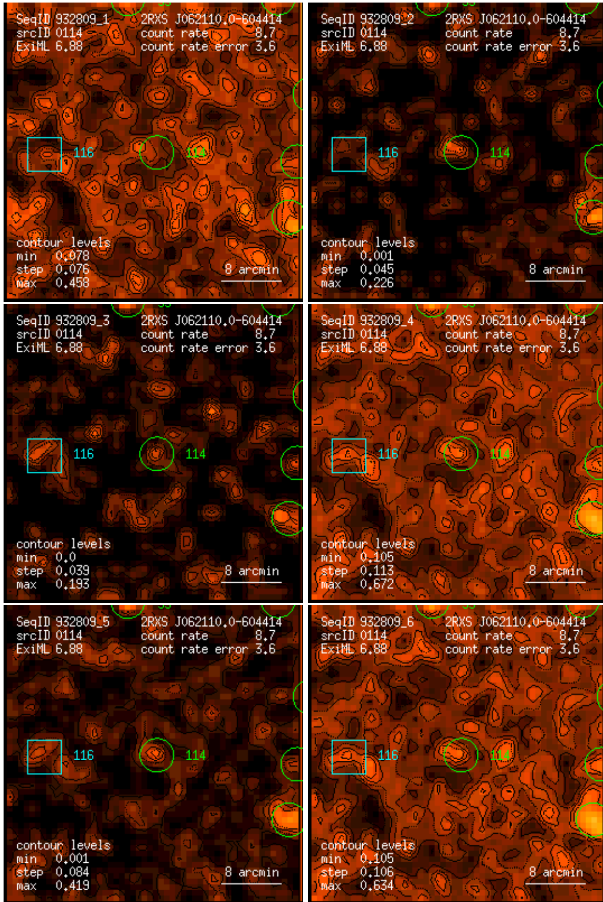
Figure 114: RASS 932809: detection 0114: band rate images, Gaussian filter: (1) PSPC channels 11 – 41, (2) 52 – 90, (3) 91 – 201, (4) 11 – 235, (5) 52 – 201, (6) 11 – 201. Broad band rates in counts/ks. Band rate contour levels in counts/ks/arcmin 2 .
