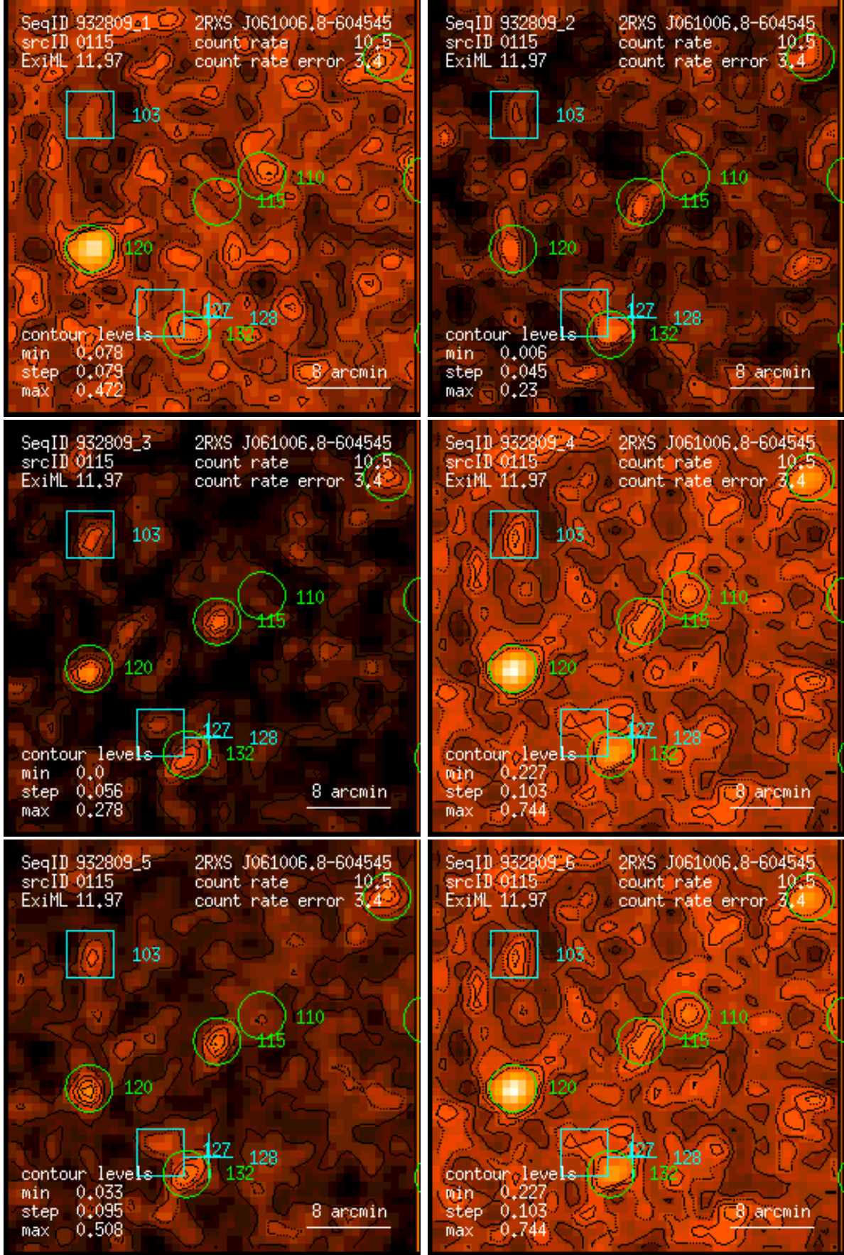
Figure 115: RASS 932809: detection 0115: band rate images, Gaussian filter: (1) PSPC channels 11 – 41, (2) 52 – 90, (3) 91 – 201, (4) 11 – 235, (5) 52 – 201, (6) 11 – 201. Broad band rates in counts/ks. Band rate contour levels in counts/ks/arcmin 2 .
