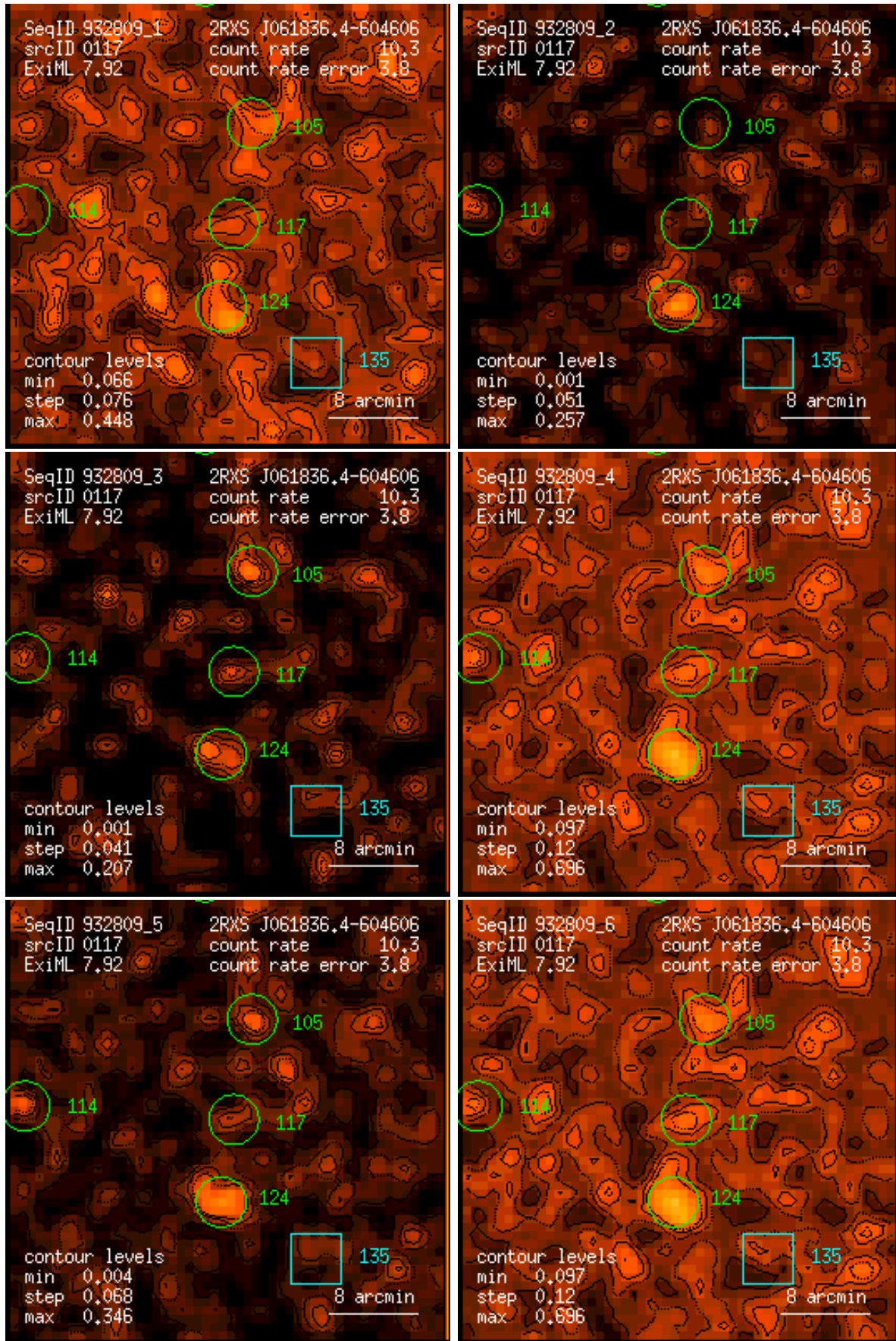
Figure 117: RASS 932809: detection 0117: band rate images, Gaussian filter: (1) PSPC channels 11 – 41, (2) 52 – 90, (3) 91 – 201, (4) 11 – 235, (5) 52 – 201, (6) 11 – 201. Broad band rates in counts/ks. Band rate contour levels in counts/ks/arcmin 2 .
