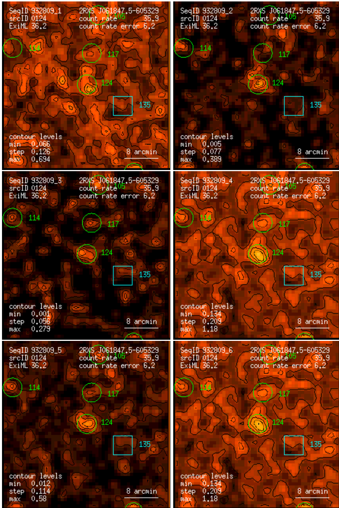
Figure 124: RASS 932809: detection 0124: band rate images, Gaussian filter: (1) PSPC channels 11 – 41, (2) 52 – 90, (3) 91 – 201, (4) 11 – 235, (5) 52 – 201, (6) 11 – 201. Broad band rates in counts/ks. Band rate contour levels in counts/ks/arcmin 2 .
