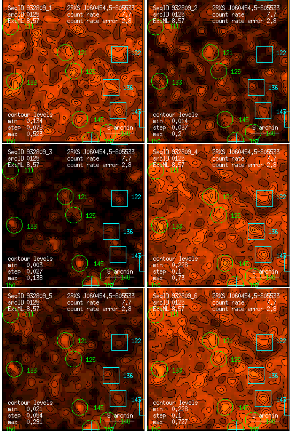
Figure 125: RASS 932809: detection 0125: band rate images, Gaussian filter: (1) PSPC channels 11 – 41, (2) 52 – 90, (3) 91 – 201, (4) 11 – 235, (5) 52 – 201, (6) 11 – 201. Broad band rates in counts/ks. Band rate contour levels in counts/ks/arcmin 2 .
