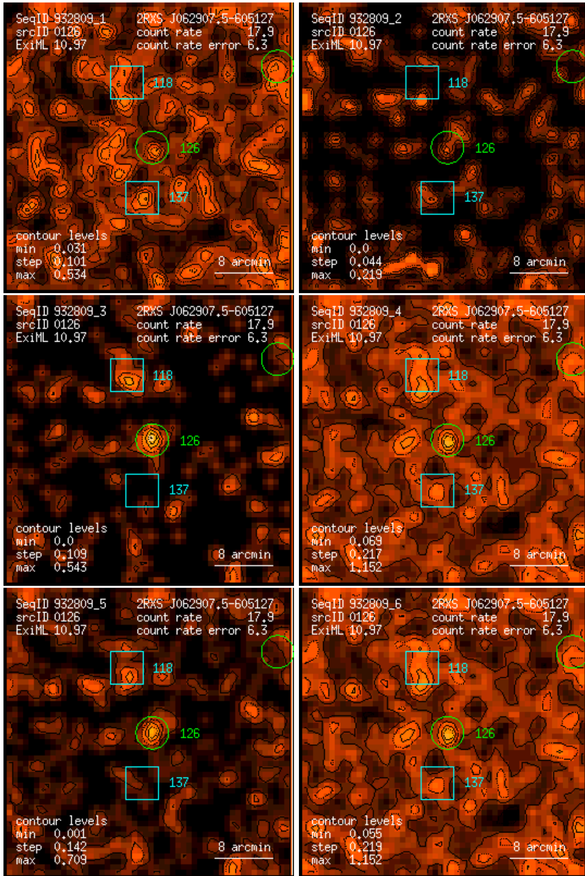
Figure 126: RASS 932809: detection 0126: band rate images, Gaussian filter: (1) PSPC channels 11 – 41, (2) 52 – 90, (3) 91 – 201, (4) 11 – 235, (5) 52 – 201, (6) 11 – 201. Broad band rates in counts/ks. Band rate contour levels in counts/ks/arcmin 2 .
